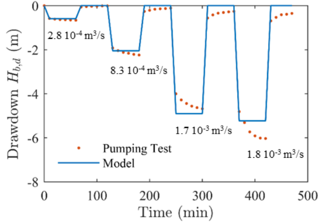
Figure 9 Drawdown measured during the pumping tests and simulated by the model
