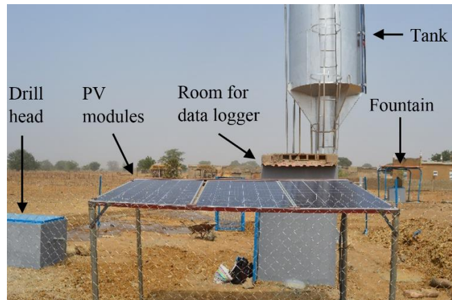
Figure 2 Picture of the PVWPS of Gogma
