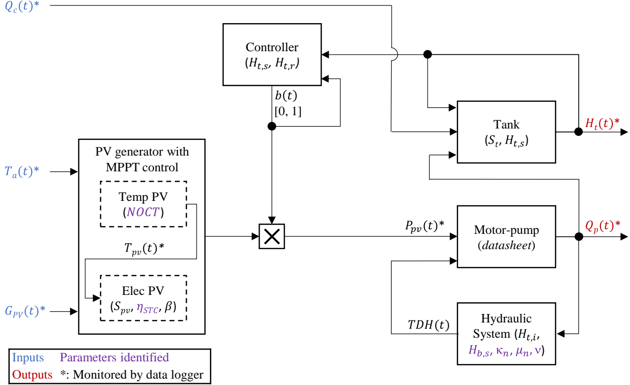
Figure 6 Block diagram of the model.
