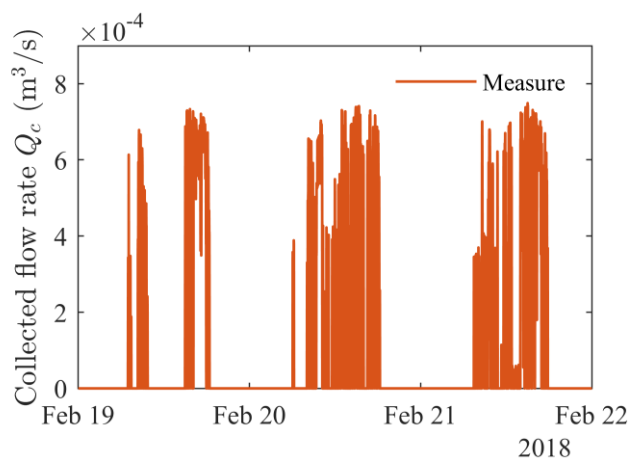
Figure 13 Temporal evolution of the water collection flow rate from local measurements (model input).
