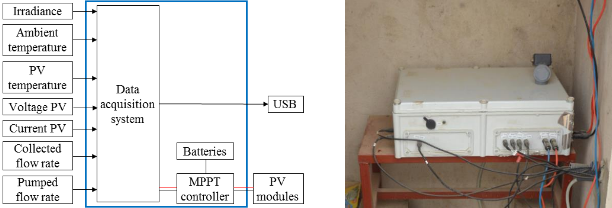
Figure 4 Data logger used for monitoring the PVWPS of Gogma
