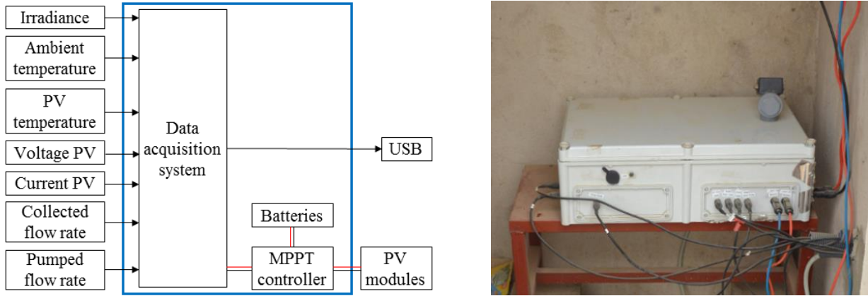
Figure 4 Data logger used for monitoring the PVWPS of Gogma
