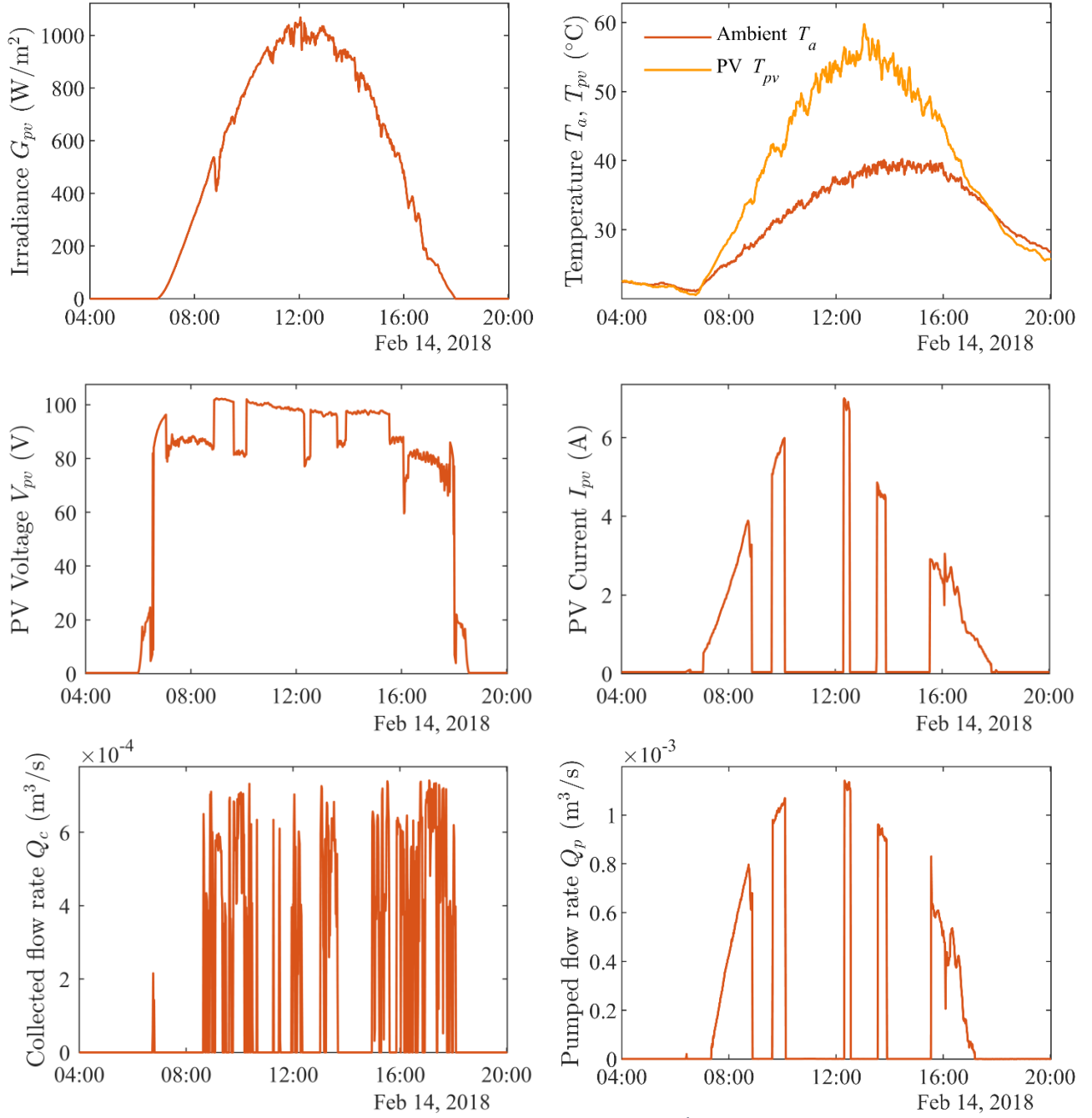
Figure 5 Data collected by the data logger on the 14 th of February 2018.
