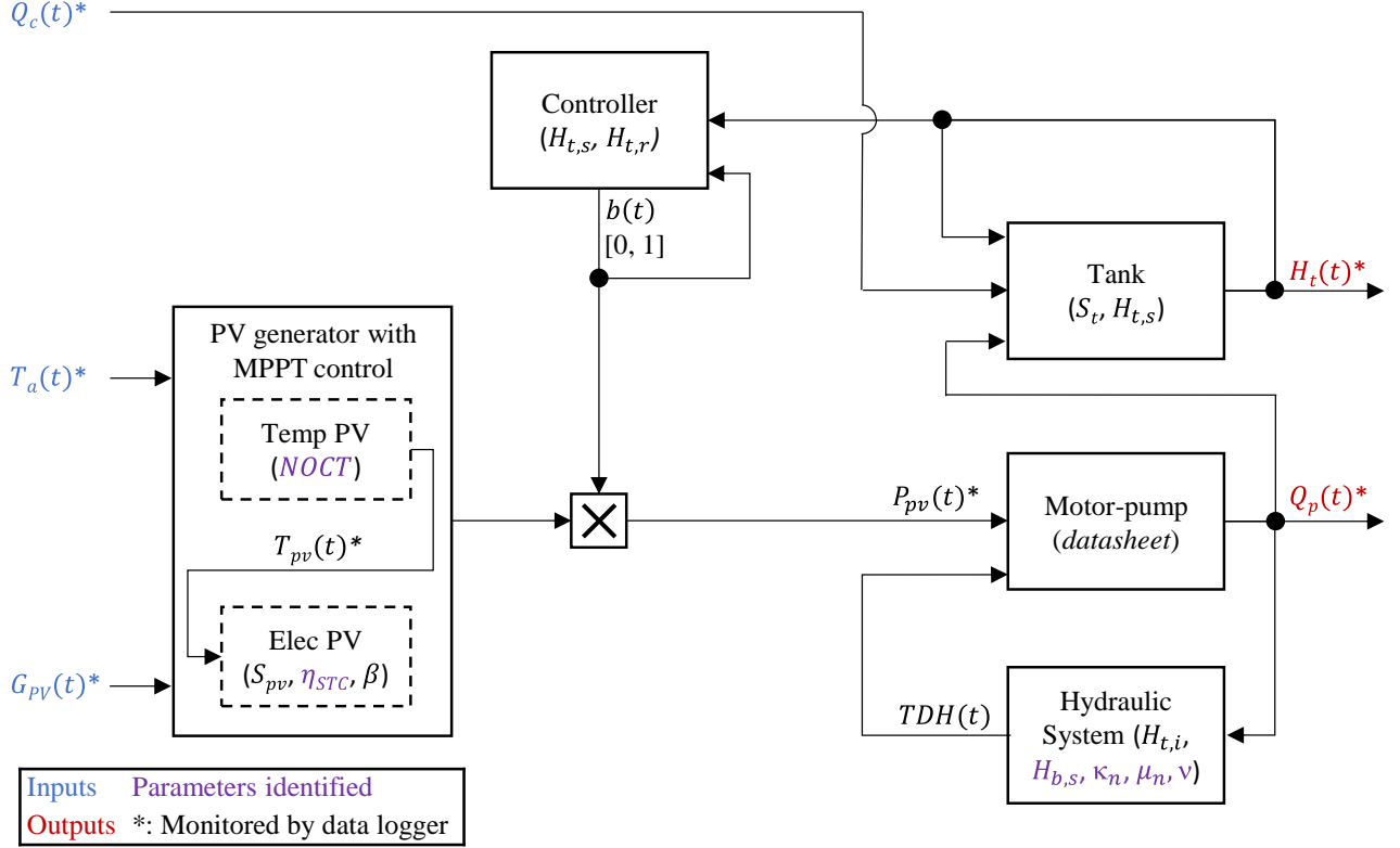
Figure 6 Block diagram of the model.
