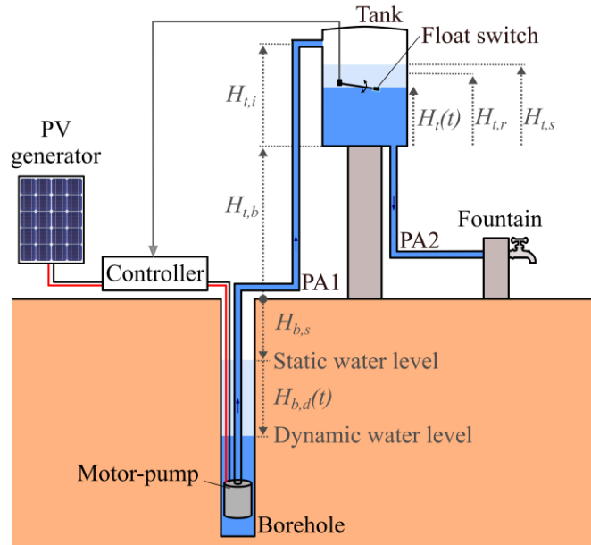
Figure 1 Architecture of the system and definition of the heights The height datum is set at the ground level so H_{b,s} and H_{b,a} are negative
