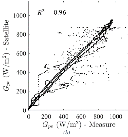
Figure 11 Irradiance on the plane of the PV modules from satellite data and from local measurements (model input) (a) Temporal evolution (b) scatter plot
