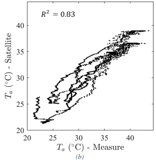
Figure 12 Ambient temperature from satellite data and from local measurements (model input). (a) Temporal evolution (b) scatter plot
