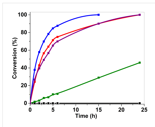
Figure 4: Monitoring over time of benzyl alcohol oxidative dehydrogenation conversion with \text{Au}_{25}(\text{SG})_{18}@\text{ZrO}_2 before calcination (black), after calcination at 200 °C for 4 hours under air, (A 200 ) (green), at 300 °C for 4 hours under air, (A 300 ) (blue), at 400 °C for 12 hours under air, (A 400 ) (red) and compared to AuNP@ZrO 2 (purple).
