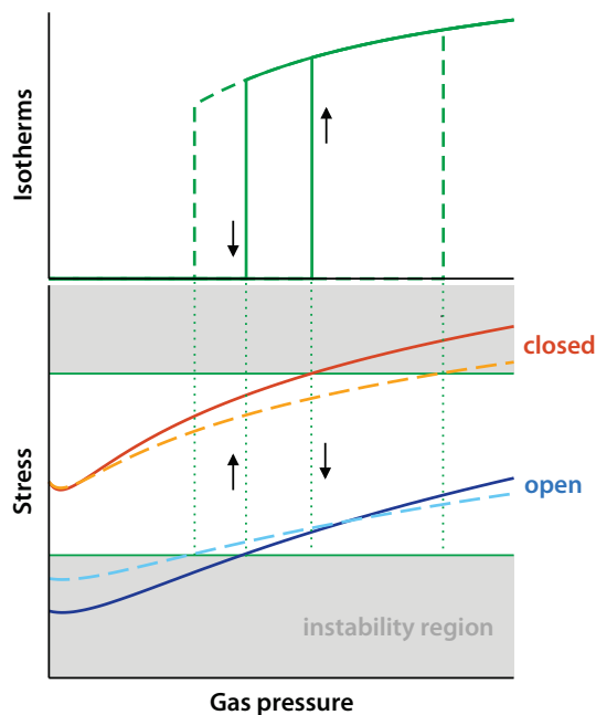
Figure 2. Gate-opening phenomenon in an isolated crystal (solid lines) and in a crystal surrounded by an elastic matrix (dashed lines). Upper panel: adsorption–desorption isotherms; lower panel: adsorption-induced stress in both phases.
