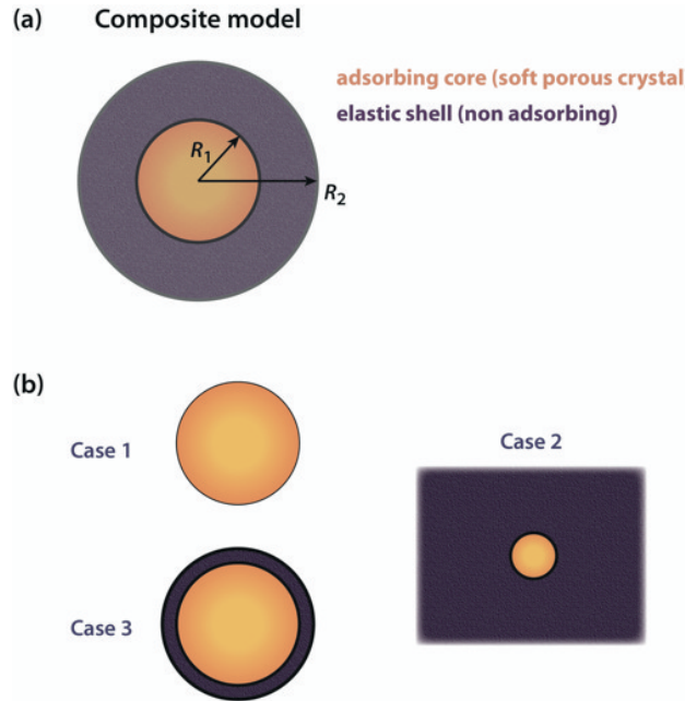
Figure 1. (a) Model system representing a composite material. (b) Three special cases of the model system: case 1, unconfined spherical adsorbent particle; case 2, adsorbent in infinite elastic matrix; case 3, spherical core-shell particle.
