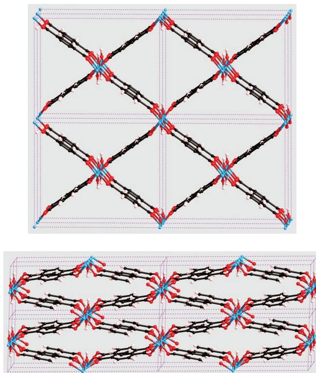
Figure 1. Representation of the metastable lp (top) and np (bottom) structures of the MIL-53(Al) material, as a 2 \times 2 \times 2 supercell viewed along the axis of the unidimensional channels.
