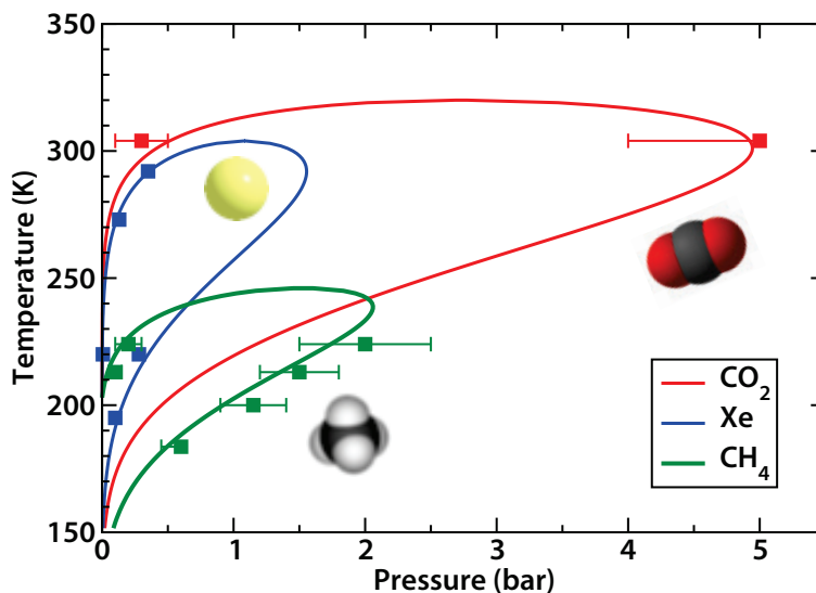
Figure 2. Comparison of the Temperature–gas Pressure phase diagrams for CO 2 (red), CH 4 (green) and Xe (blue) adsorption in MIL-53 (Al). 12 Experimental transition pressures are indicated by square symbols.
