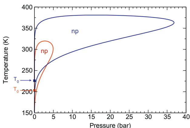
Figure 5. Temperature–CO 2 pressure phase diagrams for regular MIL-53(Al) (red) and amino-MIL-53(Al) (blue) materials. The T_0 are the equilibrium phase transition temperature between the lp and np phases at zero pressure (i.e. the empty material) for both materials. Modified with permission from ref. 11, © 2010 Elsevier Inc.
