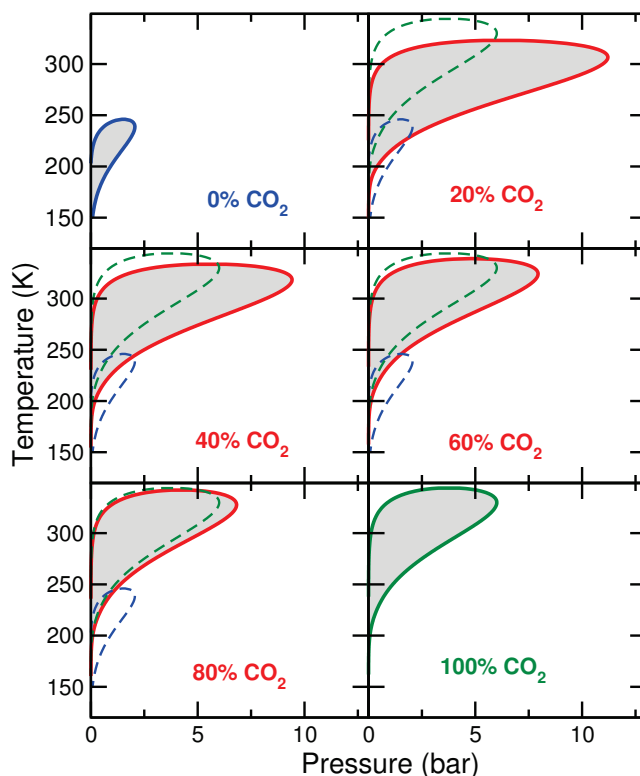
Figure 4. Temperature–pressure phase diagram of MIL-53(Al) upon adsorption of a \text{CO}_2/\text{CH}_4 mixture, with increasing \text{CO}_2 molar fraction. Dashed lines correspond to pure component diagrams: \text{CO}_2 in green, \text{CH}_4 in blue. Reproduced with permission from ref. 13, © 2011 American Chemical Society.
