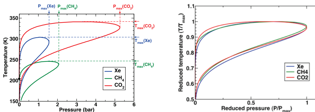
Figure 3. Left: Comparison of the temperature–vapour pressure phase diagrams for CO 2 (red), CH 4 (green), and Xe (blue) adsorption in MIL-53(Al), with the extremal temperatures and pressures marked. Right: same three phase diagrams in reduced units of (T / T_{\max}) and (P / P_{\max}) . Left figure is reproduced with permission from ref. 12, © 2010 American Chemical Society.
