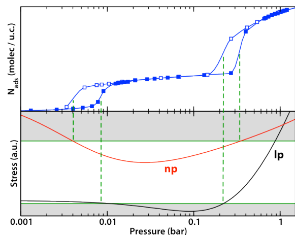
Figure 8: Xenon adsorption and desorption isotherms in MIL-53 (Al) at 220 K (upper panel) and adsorption-induced stress in each solid phase (lower panel). The stability region of both structures is indicated in white, and the unstable regions in gray. Vertical dashed lines indicate the structure transitions, which correspond to the stress in one phase crossing the stability limit. Reprinted with permission from ref. 117.
