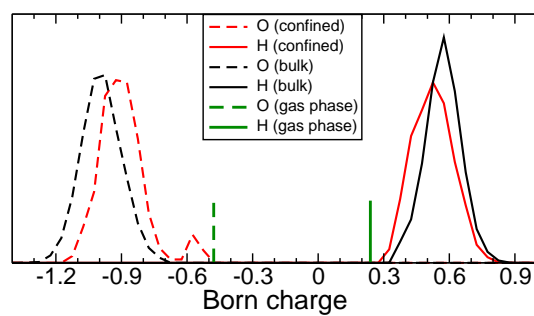
Figure 16: Distribution of partial charges of the water oxygen and hydrogen atoms according to the Born population analysis methods. The distributions were computed for water confined in an all-silica LTA (red), for bulk water (black) and for a single gas phase water molecule (green).
