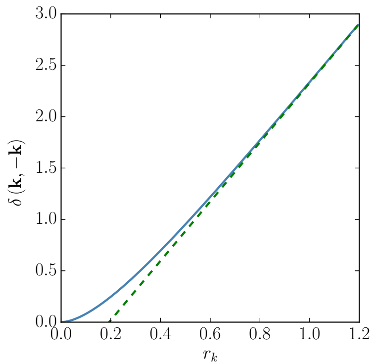
Figure 2. Quantum discord of a two-mode squeezed state as a function of the squeezing parameter r_k (solid blue line). The dashed green line represents the large r_k expansion of \delta(k, -k) —figure taken from Ref. [23].
