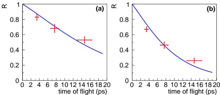
Fig. 4. Fit of the R ratio as a function of time of flight between target and degrader using the Bateman equations for the 2^+ (a) and 4^+ (b) states of ^{88}\text{Kr} .
