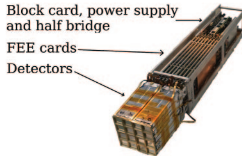
Fig. 1. – Picture of a FAZIA block. The detectors and the front-end electronics are highlighted.
