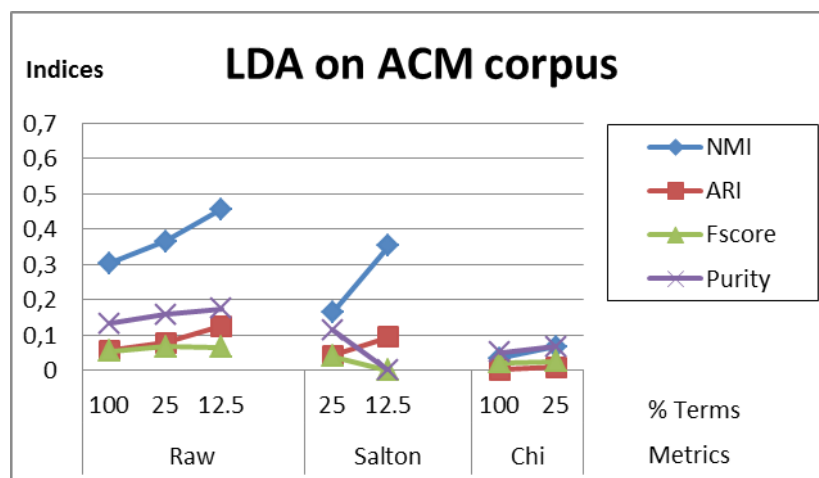
Figure 7: LDA on ACM corpus
