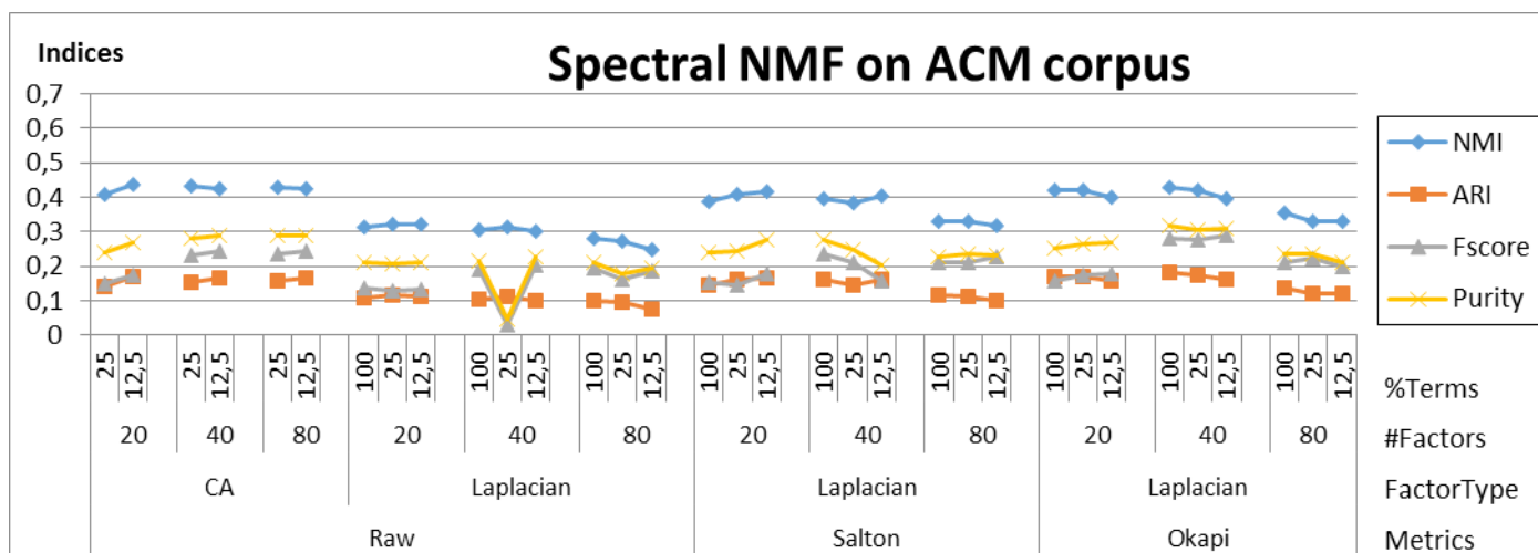
Figure 13: Spectral Non-negative Matrix Factorization clustering on (un-)weighted ACM corpus
