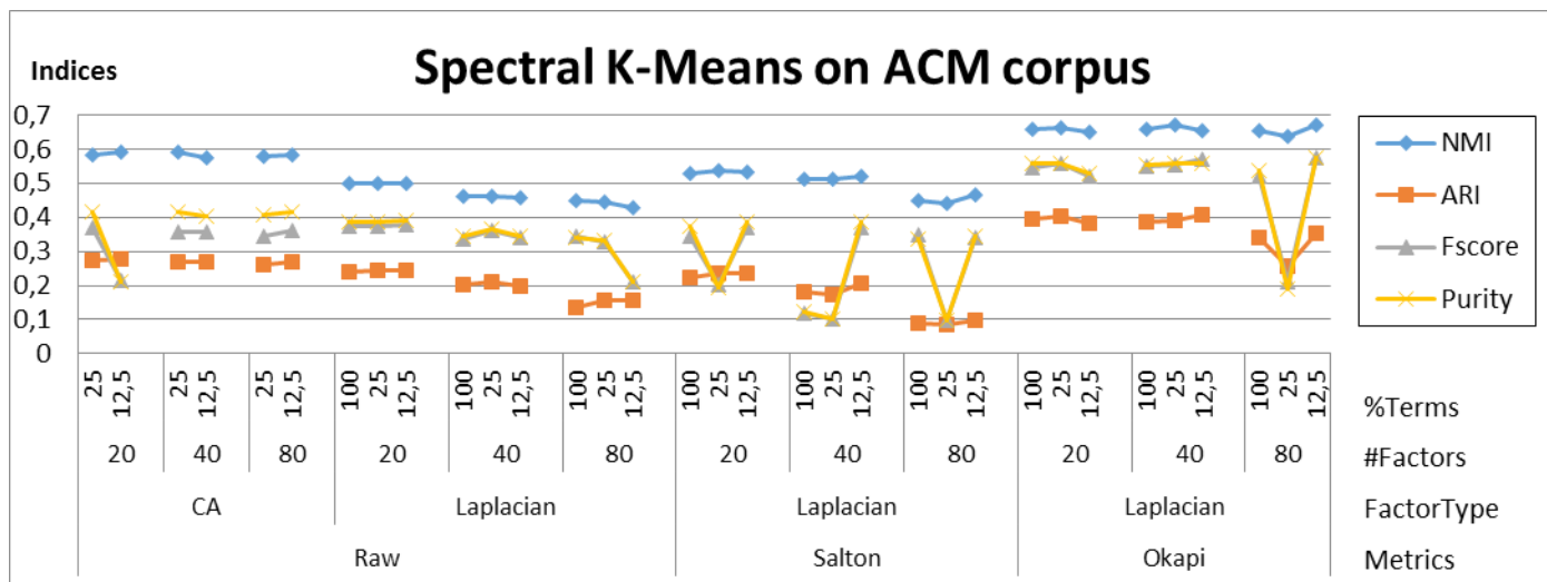
Figure 12: Spectral K-means Clustering on ACM corpus
