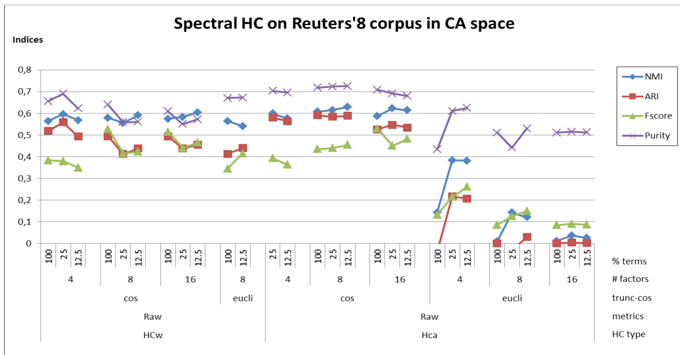
Figure 18: Spectral Hierarchical Clustering on Re8 corpus in Correspondence Analysis factor space (cosine distance) HC-average is clearly a bad option in raw CA space, but a very good one using cosine distance in this dataspace.
