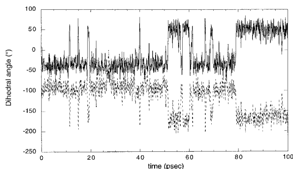
Figure 4. Dynamical behaviour of the \chi_1 (continuous line) and \chi_3 (broken line) torsional angles of the Glu62 side-chain, during a 100 ps time span starting at the end of the Ca 2+ \rightarrow Mg 2+ transformation within the EF-3 site of parvalbumin. The \chi_2 angle remains rather constant around a -170^\circ value (data not shown).
