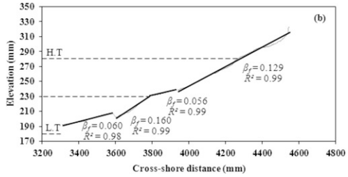
Fig. 8 Dynamic beach profiles measured by optical method during (a) rising tide and (b) falling tide at the equilibrium state for Test 4. The solid line refers to the foreshore beach slope ( \beta_f ). The dashed lines refer to the still water level at low (L.T), mean and high (H.T) tides.
