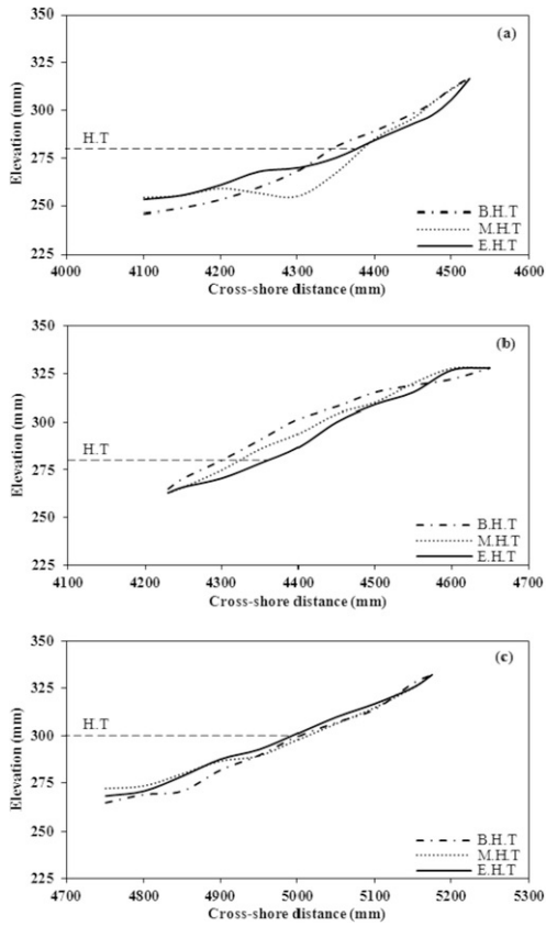
Fig. 9 Morphological evolution of the upper part of the beach during high tide for the beginning (B.H.T), middle (M.H.T) and end (E.H.T) of the phase for (a) Test 4, (b) Test 5.a and (c) Test 6. The dashed line refers to the still water level at high tide (H.T).
