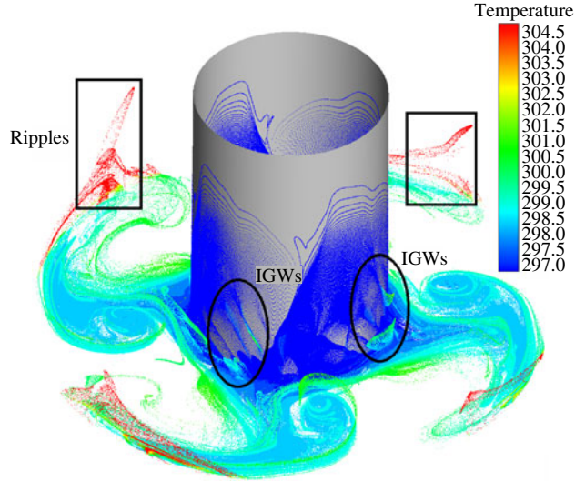
FIGURE 6. (Colour online) The HOC model. Snapshot of the tracks of particles 150 s after release. Four million particles are uniformly released in a (\phi, z) plane at radius r = 45.15 mm (supplemental movies 3 and 4). Particles are coloured by the local temperature: blue (red) colour = cold (hot) temperature (K). The locations of IGWs at the inner sidewall (ripples at the outer one) are highlighted by ellipses (rectangles).
