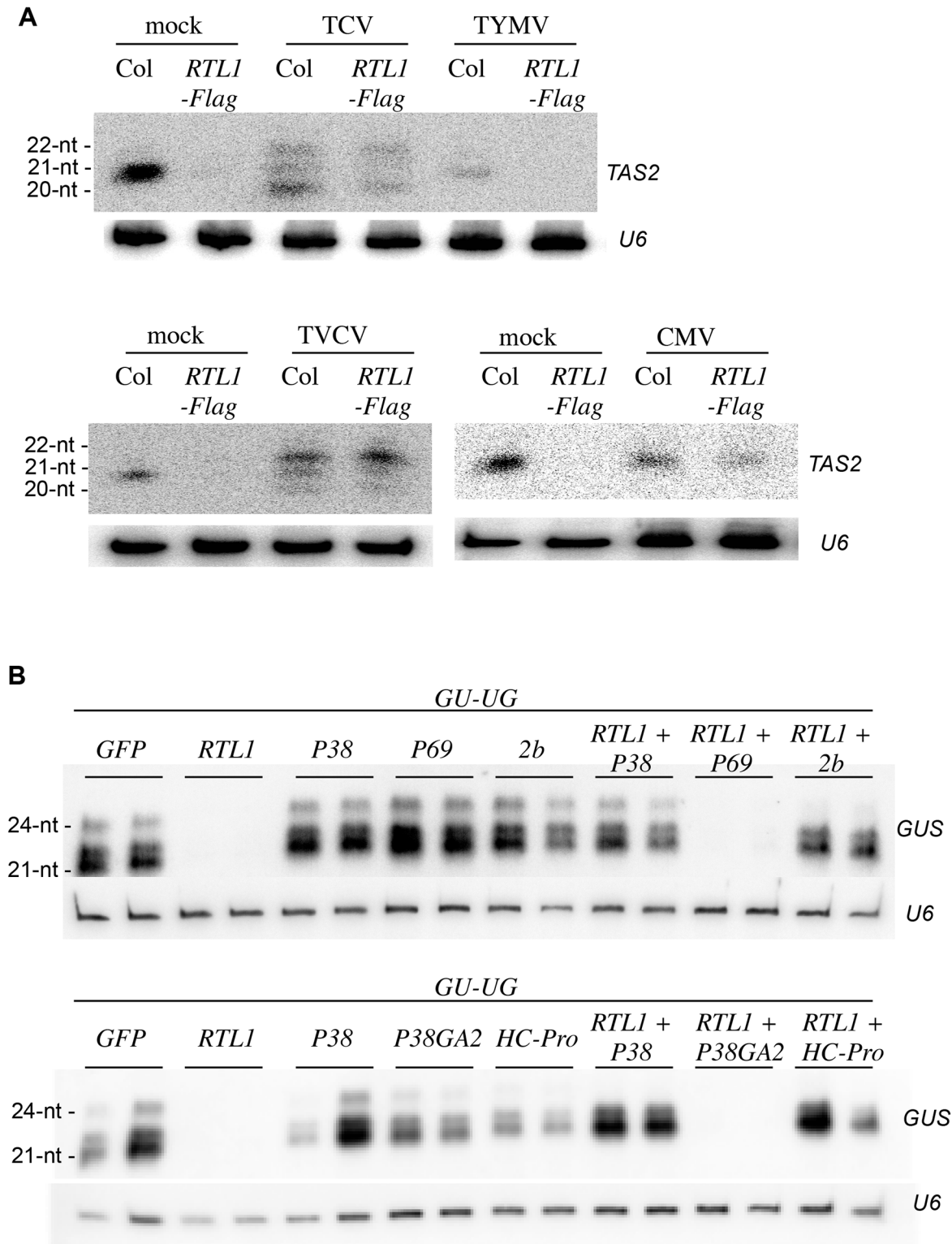
Fig 7. RTL1 activity is suppressed by VSRs. A ) RNAs extracted from water (mock)- or virus inoculated wild-type (Col) and 35S: RTL1-Flag ( RTL1-Flag ) plant #2 were hybridized with a TAS2 probe and U6 as a loading control. B ) N. benthamiana leaves were infiltrated with a 35S: GU-UG construct ( GU-UG ) together with either a 35S: GFP control ( GFP ), a wild-type 35S: RTL1 construct ( RTL1 ), a 35S: VSR construct ( P38 , P38GA2 , P1/HC-Pro , 2b , or P69 ), or a mix of the 35S: RTL1 and 35S: VSR constructs. LMW RNAs were hybridized with a GUS probe and with U6 as a loading control.
