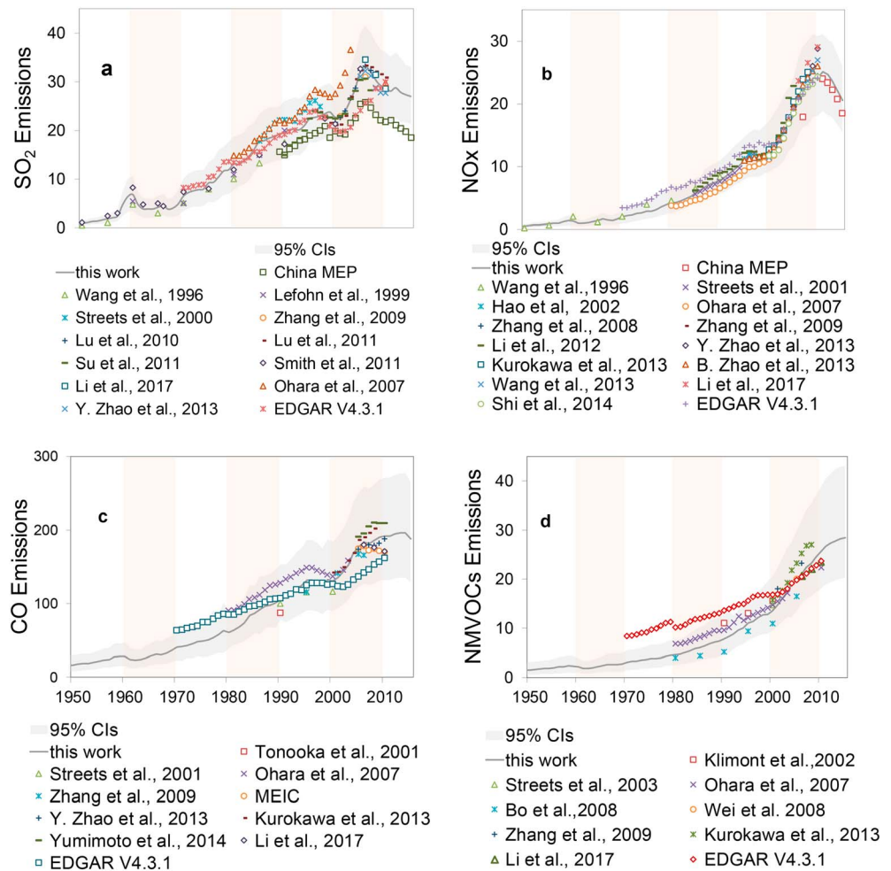
Figure 6. Comparison among multiple estimates of Chinese air pollutants emissions: (a) SO 2 ; (b) NO x ; (c) CO; (d) VOCs. The solid lines indicate our result, and gray areas indicate the uncertainty of our results (95% CIs). Other points indicate the estimated emissions from the China MEP or other studies. CI = confidence interval; MEP = Ministry of Environment Protection; NMVOC = nonmethane volatile organic compound.
