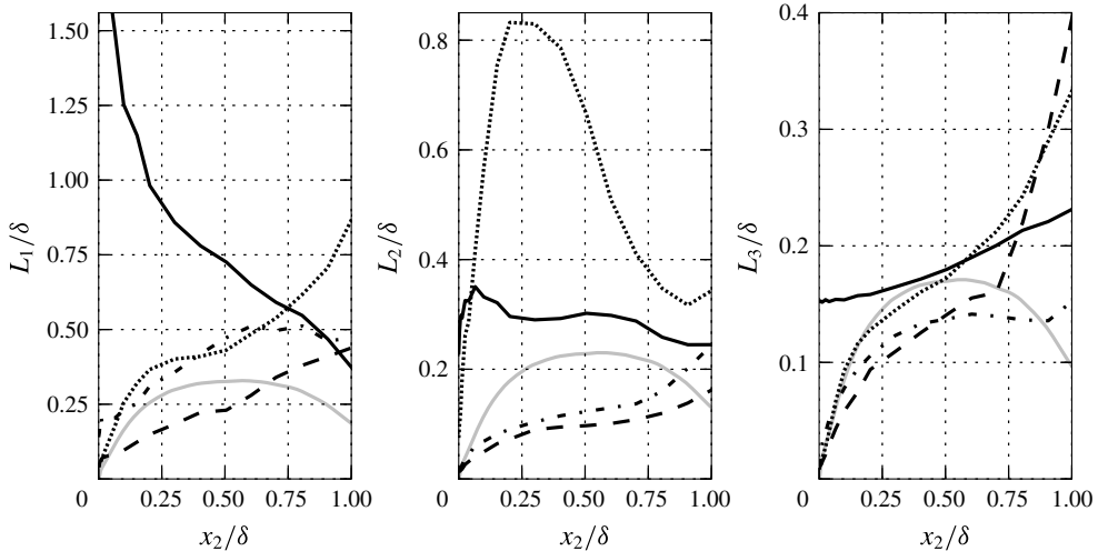
FIGURE 7. Correlation lengths for the EAM scaled in outer units: — (black), C_{11} ; ---, C_{22} ; - · - ·, C_{33} ; · · · · ·, \tilde{C}_{12} . The grey lines represent equivalent correlation lengths ( L_i \equiv 0.54\gamma_i L_u ) for the SAM for C_{11} .
