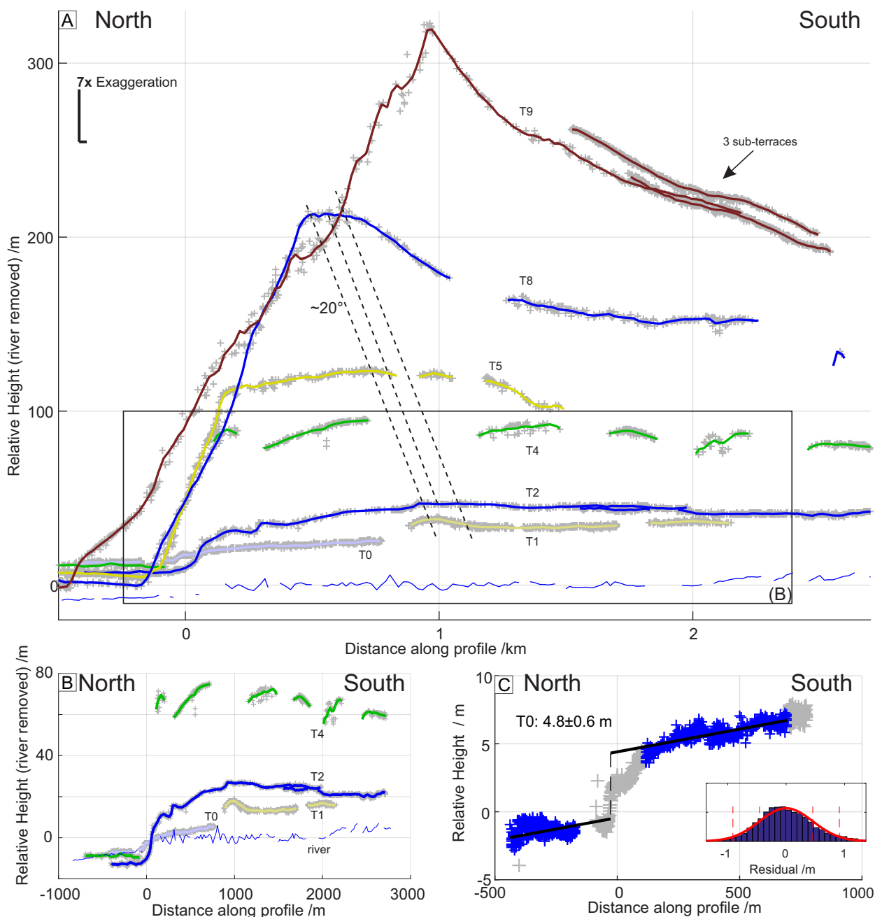
Figure 7. (a) Long profiles along all of the terraces, collapsed onto an azimuth of 80°. All of the terraces show an increase in displacement relative to modern river level towards the basin, suggesting the fault dip flattens upwards.(b) Profiles across the lowest four terraces at the Rc2 catchment show a broad warping. It is unclear whether T1 and T0 are the same terrace. (c) Profile across the unique low scarp (T0), measuring a vertical offset of ~4.8 m at the fault trace (inset shows histogram of residuals).
