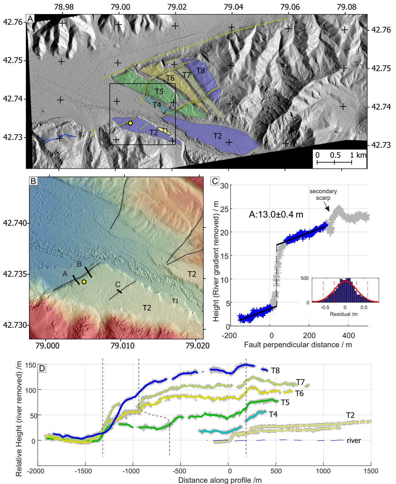
Figure 8. (a) Map of the Basharin site, highlighting the series of terraces observed. Labels correspond to the correlated terraces at other sites (§2.2). (b) Zoom near the scarp, showing the location of the three shallow hammer seismic refraction/reflection lines across the scarps, and the sampling pit location. (c) A topographic profile across the scarp in the most recent displaced terrace (T1), in the vicinity of seismic reflection profiles A and B. The inset shows the histogram of residuals. (d) Long profiles through the flight of terraces collapsed onto an azimuth of 070^\circ , show displacements of up to 150 m relative to the modern river channel; the older terraces mark fault displacement in several locations (dashed lines). The older terraces with greater maximum displacement show more displacement further north, while the more recent terrace only shows displacement on the southern fault strand.
