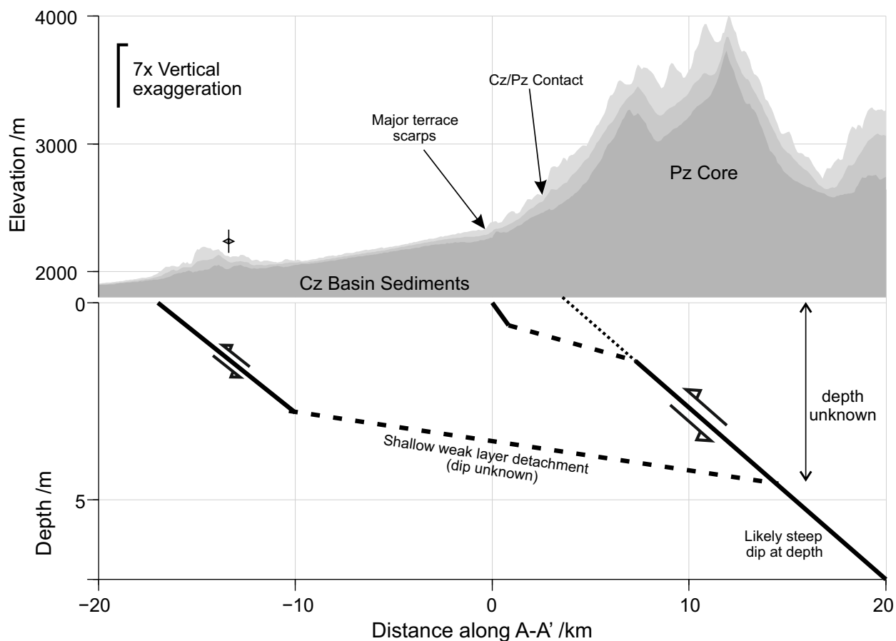
Figure 15. Conceptual model of the Karkara Rangefront Fault (KRF) and the Kegen Basin Fold (KBF). The KBF has a width of 6.5 km, suggesting that it is underlain by a ramp that shallows into a detachment at several kilometres depth, and which we interpret to extend southwards to connect with the KRF. The active trace of the KRF is sited north of the Cenozoic-Palaeozoic bedrock contact. The deformation of terraces in the hanging wall of the fault suggest that it shallows into a detachment at only 1-2 km depth, which is also likely to splay from the main fault zone.
