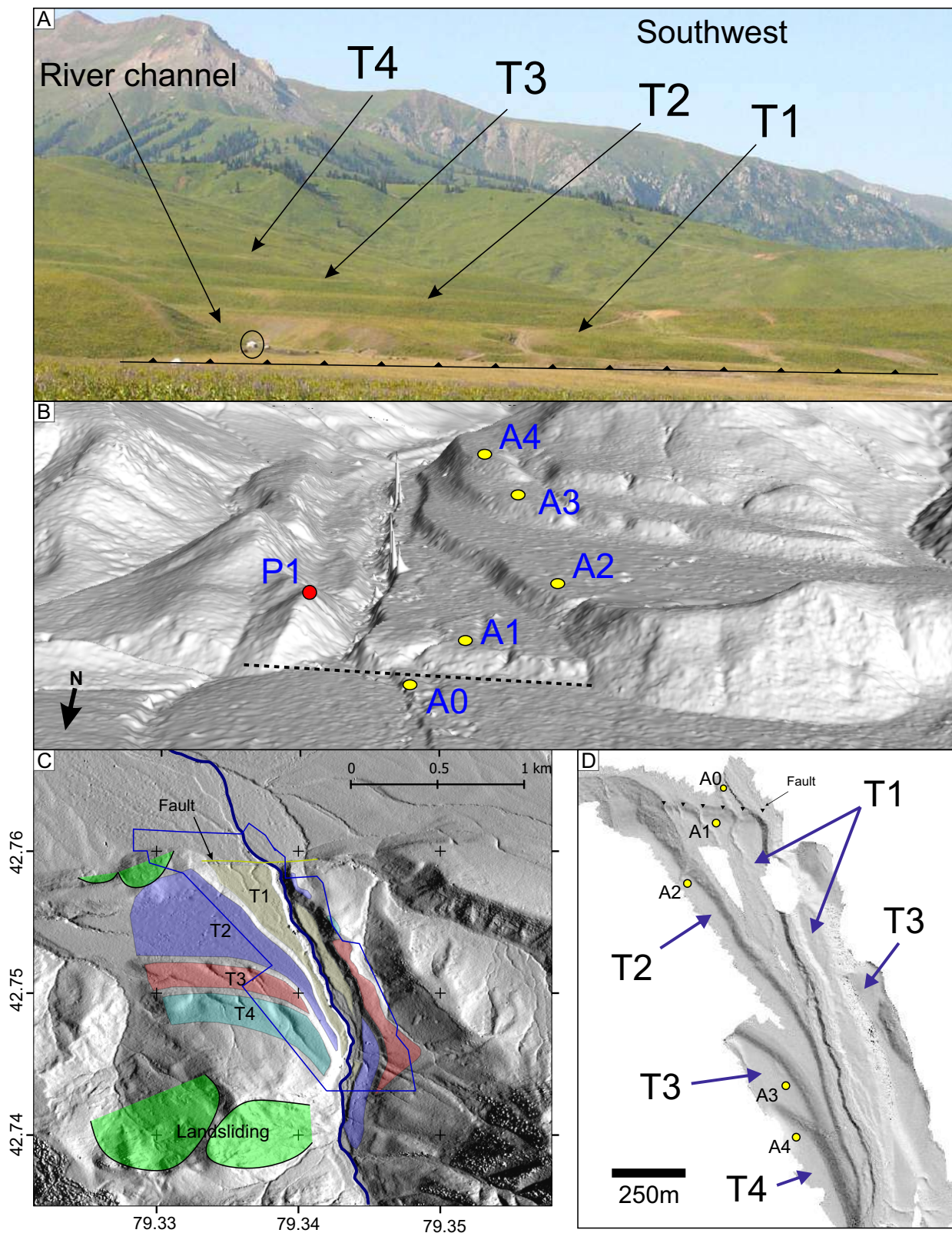
Figure 3. (a) Overview of the stepped terraces, T1-4, with the fault in the foreground, yurt circled for scale. (b) Perspective view looking south at the flight of terraces, based on shaded relief of the Pléiades 2 m DEM. Sampling sites are marked as yellow dots. Red dot marks location of photo in Figure 5. 2x vertical exaggeration. (c) Map of the terraces at Rc1. T1-4 shown as coloured polygons with colours consistent with the terraces shown in later figures. Green line marks the fault surface trace in the most recently abandoned terrace. Landslides shown as green polygons. Blue outline shows the extents of the SfM survey in (d). (d) Shaded relief of the 30 cm SfM DEM, with terraces and sampling locations labelled.
