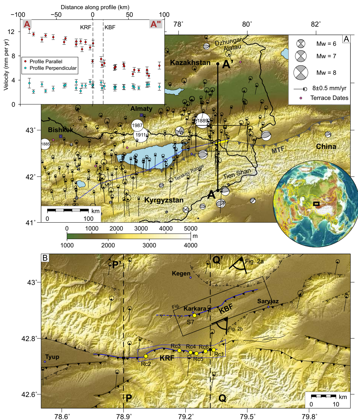
Figure 1. (top) An overview of the NE Tien Shan. Historic earthquakes of M > 6 are shown as open circles, and focal mechanisms show modern instrumental earthquakes of M > 6 from the global centroid moment tensor (GCMT) catalogue. GPS velocity vectors are from Zubovich et al. (2010) and ellipses indicate the 95% confidence interval. The blue line represents the discrete step in the northwards regional GPS velocities identified by England & Molnar (2015). (inset) GPS velocity vectors over a swath width of \pm 40 km projected on to the line A–A'. Dashed line indicates the surface fault location. Error bars indicate the 95% confidence interval. Modified after Mackenzie et al. (2015). (bottom) Inset showing the Karkara Range front (KRF), the Kegen Basin Fold (KBF), and the individual study sites Rc1–3. Blue outline shows the extents of the stereo Pléiades derived DEM. Profiles P–P' and Q–Q' are the two profiles taken through the regional GPS velocity field, modelled to estimate the fault creep rate (Figure 14).
