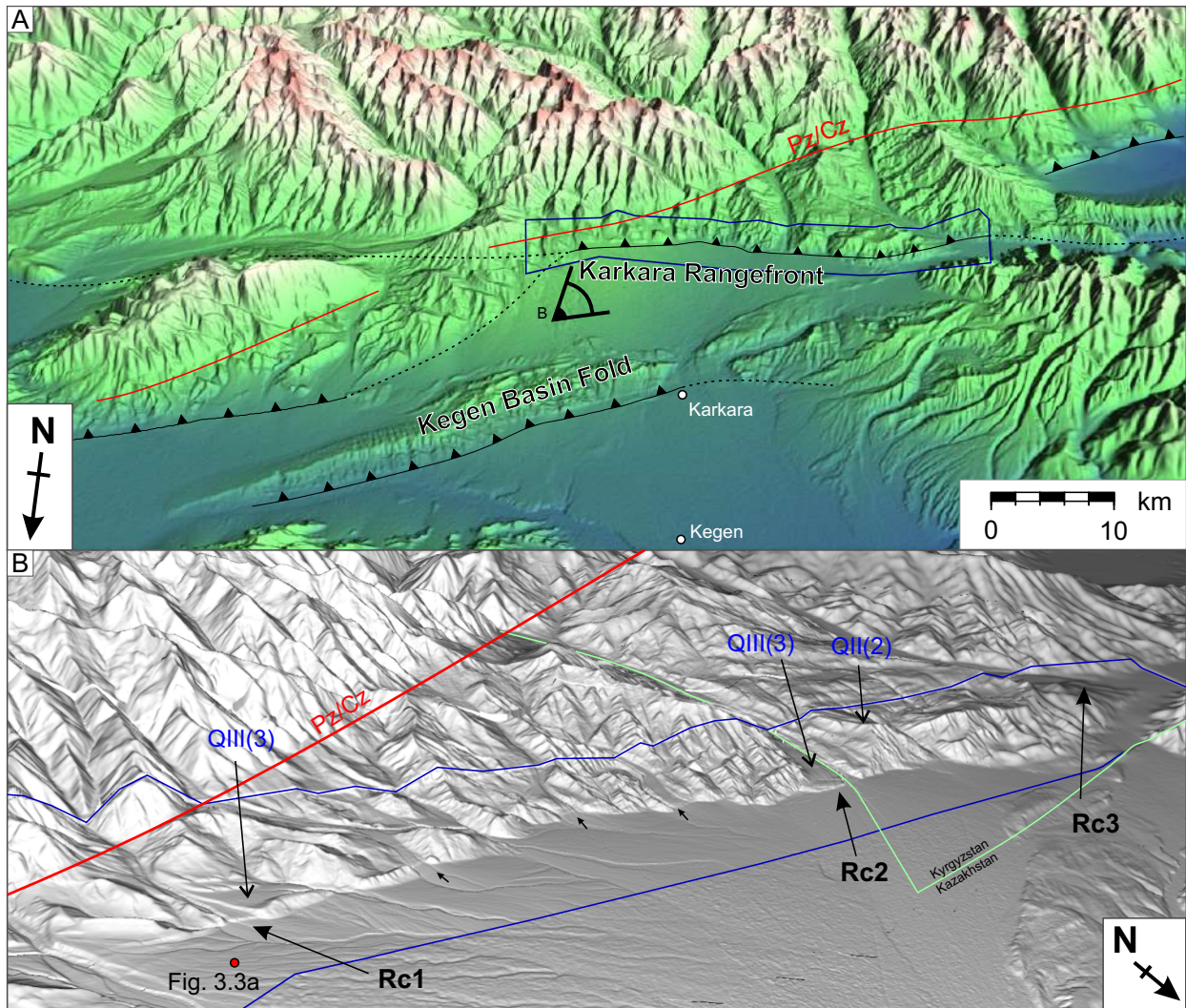
Figure 2. (a) Perspective view of the Terskey northern rangefront, showing the major structures studied here. Basemap elevation data from the SRTM 1-second dataset. 2x vertical exaggeration. Red line indicates the Palaeozoic–Cenozoic contact at the surface for the Karkara Rangefront. (b) Perspective view looking SW along the KRF, from the Pléiades derived DEM on top of the AW3D30 DEM (Takaku et al. 2014), showing the individual river catchments studied. Minor arrows indicate the catchments described in Supplement S2. Blue lines outline of the high resolution dataset.
