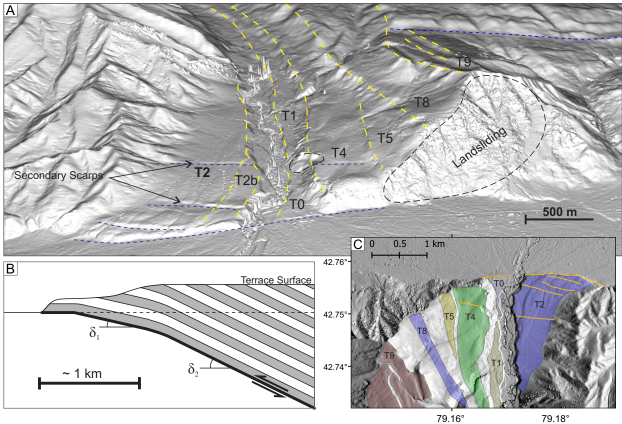
Figure 6. (a) Perspective view of the DEM at the border site at Rc2 (looking S, illuminated from viewpoint). The background low resolution DEM is from the AW3D30 dataset, in which the larger terraces are still visible. Terrace riser tops are highlighted with yellow dashed lines. Fault scarps are shown as blue dashed lines. (b) Hypothetical model of the shallow subsurface based on the terrace deformation (see Figure 7) with indicative horizontal scale included. The fault is likely to flatten into a detachment at depths greater than represented here, as inferred from southward-directed tilting of the terraces over distances of greater than 1 km. (c) Map of the terraces observed at Rc2, on top of shaded relief from the Pléiades DEM (illuminated from the East). Terrace polygon colours are consistent with those correlated at the other catchments.
