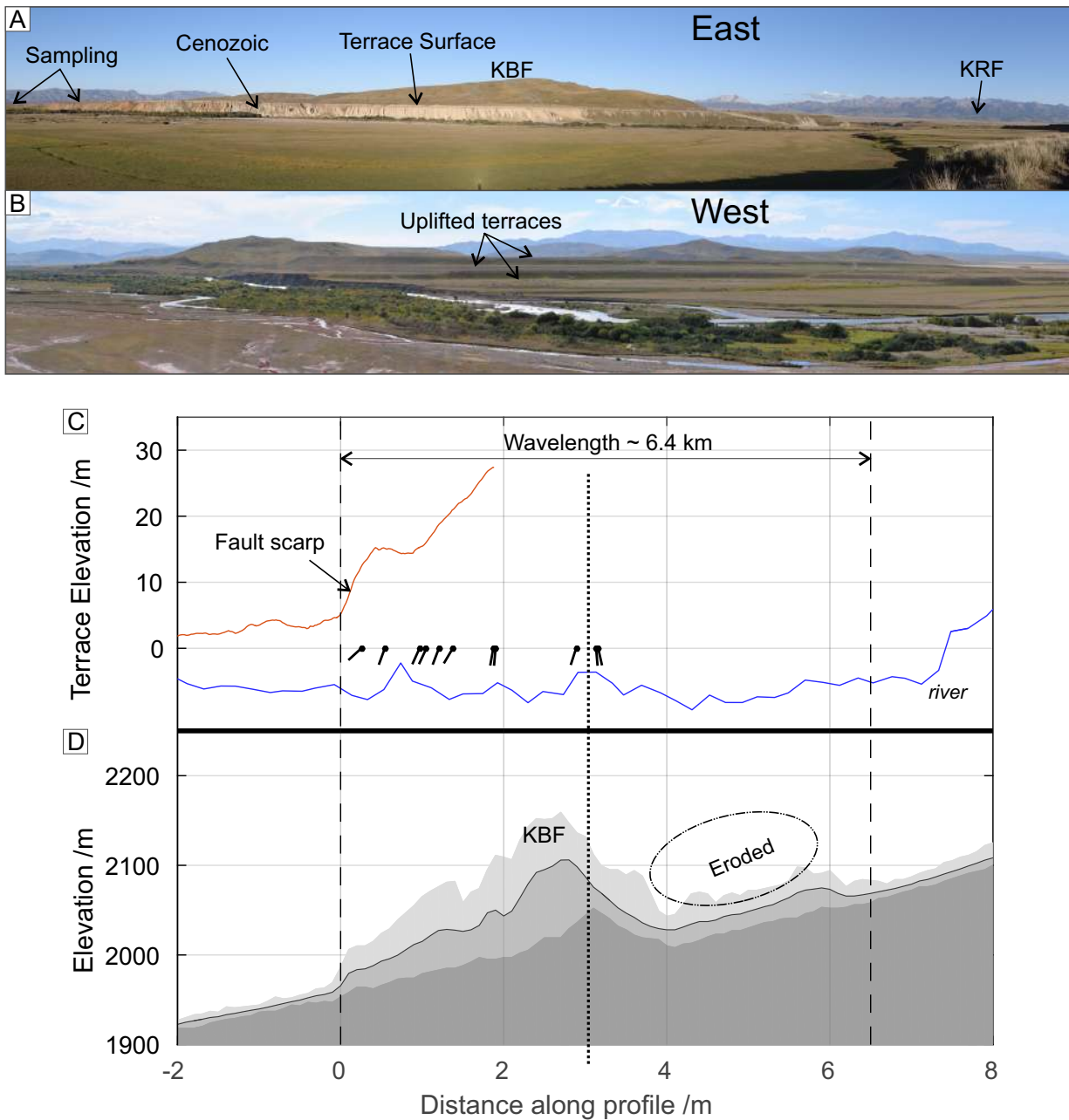
Figure 12. (a) Photograph looking east across the Karkara river to the long continuous terrace surface on the eastern side. The terrace consists of a thin gravel layer lying unconformably on steeply dipping Cenozoic sediments. Behind the terrace, the profile of the fold can be seen. (b) Photograph looking west across the Karkara river to the flight of terraces on the western side. (photo locations in Figure 11). (c) Long terrace profile with kinematic GPS along the terrace warped by folding is shown in red. The present river gradient, estimated from SRTM, has been removed from the profiles. The residuals to a linear fit to the present river channel over the wavelength from the fold is shown in blue. The apparent bedding dips are marked in black, showing a clear change from north dipping to south dipping at \sim 3 km from the fault trace (markers not scaled to the vertical axis). (d) Cross section through the minimum, mean and maximum topography across the fold in the swath profile shown in Figure 11.
