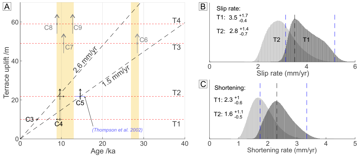
Figure 10. (a) Plot of uplift against age for the terraces at Rc1. Points in black represent those used to estimate uplift rates. Grey points represent anomalously young ages, possibly due to accelerated soil development or excessive groundwater in the post-LGM period. Yellow highlight indicates the two short periods that capture the majority of the dated samples. Horizontal dashed lines represent the estimated minimum terrace uplifts relative to the modern river level. (b-c) Monte-Carlo simulation generated PDFs for the shortening rate and slip rate based on the uplift rates for T1 and T2.
