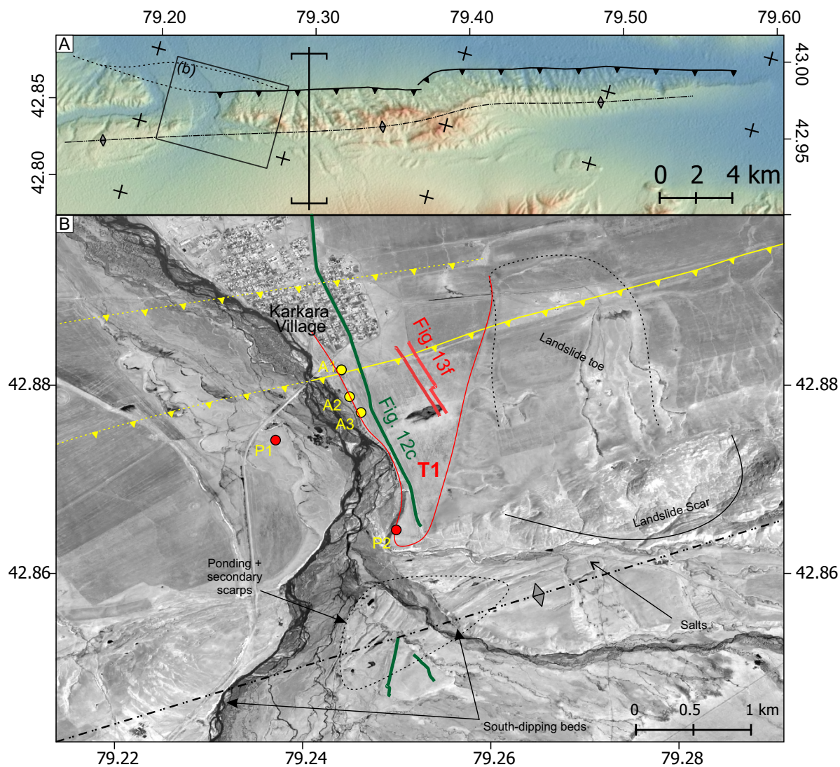
Figure 11. (a) Map of the Kegen Basin Fold, which runs approximately NE-SW across the Kegen Basin. The estimated fold axis is shown, along with the mapped fault at the surface along the northern edge of the fold. B–B' marks the location of the topography swath profile in Figure 12 (b) Map of site Q7, where the Karkara River cuts the Kegen fold. Basemap is 1 m resolution panchromatic Kompsat-2 imagery. Locations of the GPS profiles are shown as red and green lines. Sampling sites are shown as yellow dots, and the locations of the photos in Figures 12a,b, 13a, are shown as red dots.
