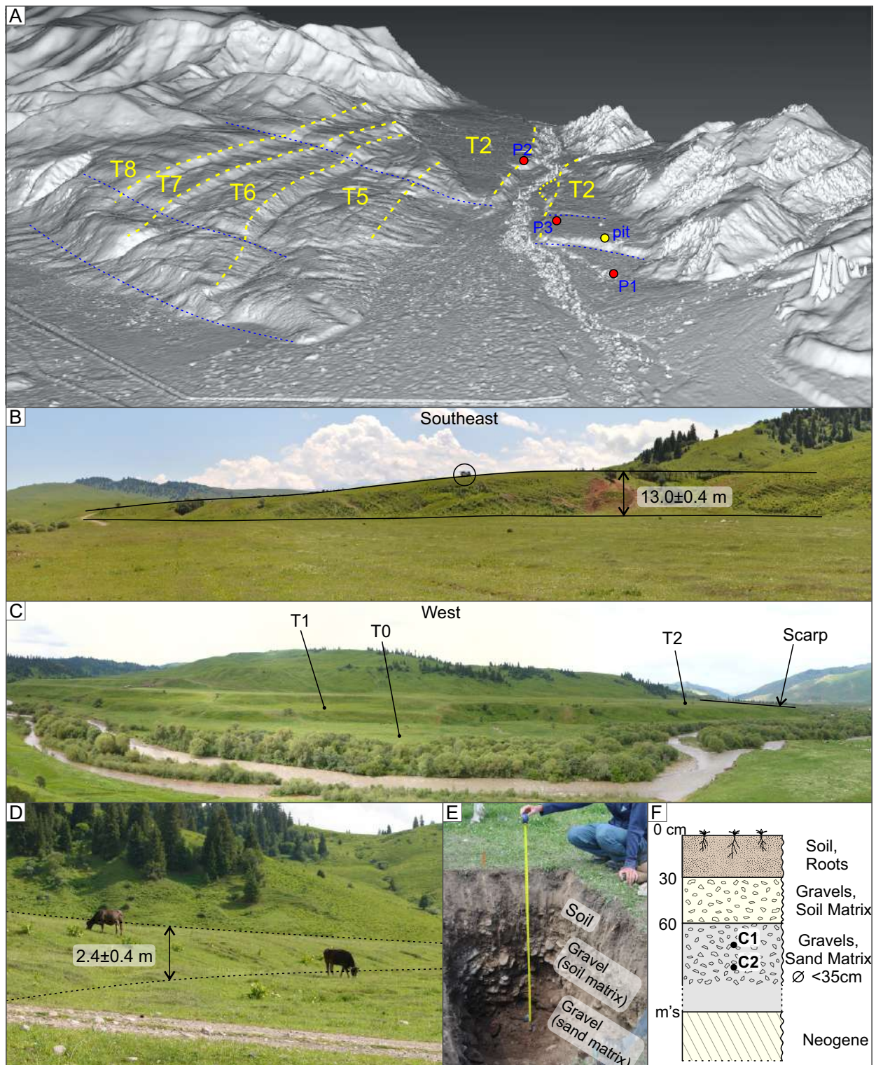
Figure 9. (a) Perspective view of the flight of terraces at Rc3. Note the tilting of the terraces away from the river channel. P1, P2 and P3 mark the locations of the photos in (b), (c) and (d) respectively. Blue dashed lines mark fault scarps. (b) Panoramic view (3 photos stitched in cylindrical projection) of the fault scarp in the T2 terrace surface, with an offset of \sim 13 m. Car for scale. (c) Panoramic view of the terraces on the western bank (5 photos, stitched in stereographic projection). (d) The smaller secondary scarp (cows for scale), \sim 400 m from the main scarp in the terrace surface of T2 has an offset of \sim 2.4 m. (e) Sampling pit in the T2 surface. (f) Stratigraphy of the T2 terrace surface. Both radiocarbon samples came from within the gravels with a sand matrix. The presence of Neogene sediments at several metres depth is inferred from outcrops in the present river bed and the seismic reflection profile.
