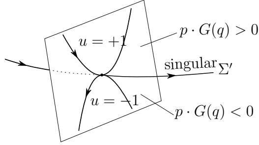
Figure 2: Fold case in the hyperbolic case in dimension 2 and the turnpike phenomenon
