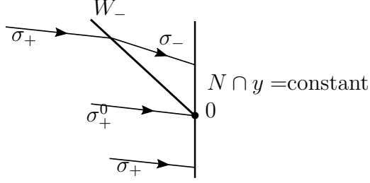
Figure 9: Parabolic case: \hat{u}(0) \in ]-1, 1[ .
