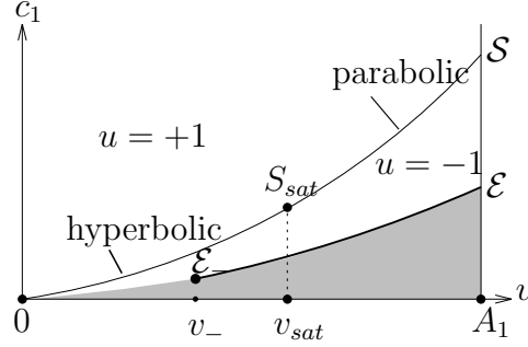
Figure 16: Stratification of the manifold N for \alpha > 1 . Non-accessible points are in the filled region and on the dotted-line of \mathcal{E} and points on \mathcal{E}_- are accessible.
