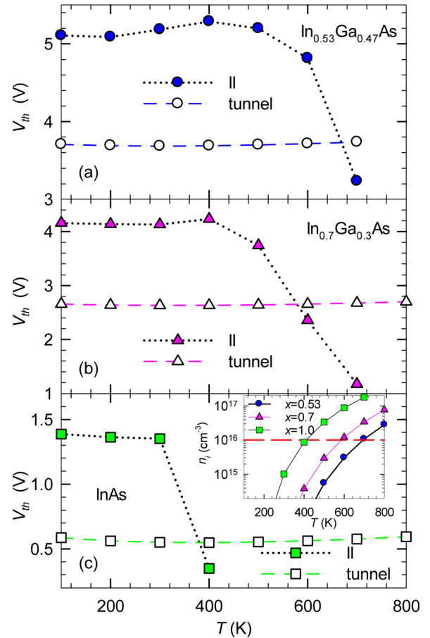
FIG. 3. MC values of V_{th\_II} and V_{th\_tunnel} as a function of T for (a) \text{In}_{0.53}\text{Ga}_{0.47}\text{As} , (b) \text{In}_{0.7}\text{Ga}_{0.3}\text{As} , and (c) InAs 100 nm PIN diodes. Inset of Fig. 3(c): n_i as a function of T for the three materials.
