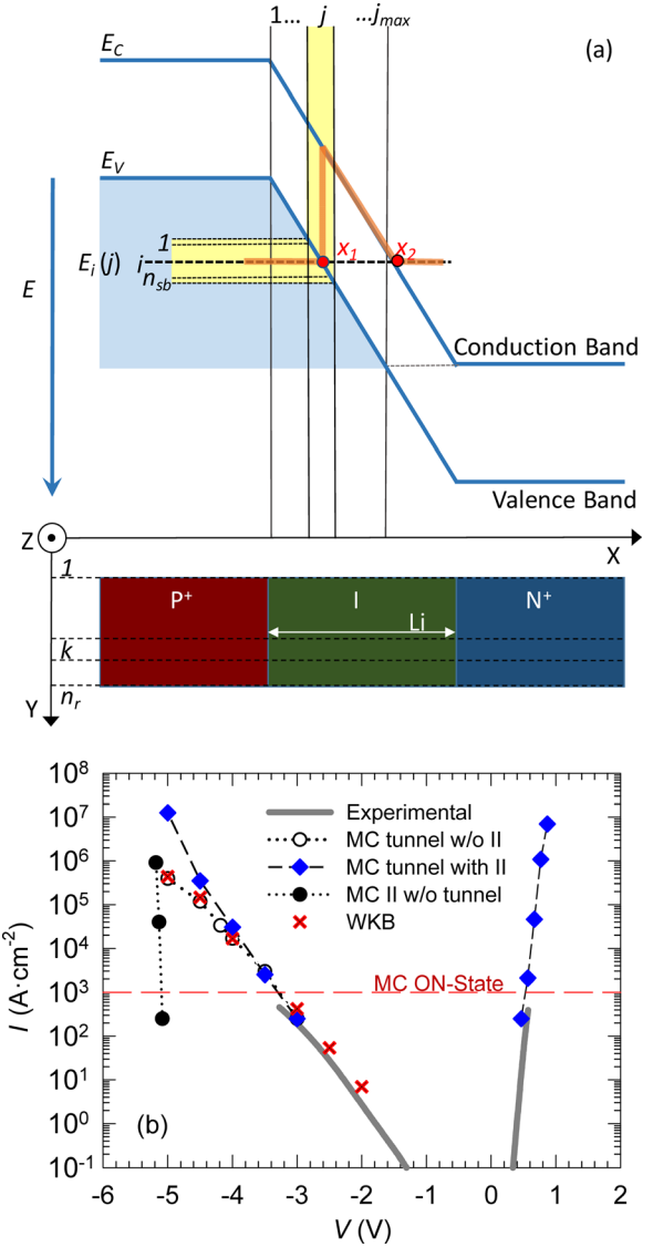
FIG. 1. (a) Schematic drawings of the energy bands with the discretization of the 2D MC domain and energies for the calculation of the tunneled charge ( x_1 and x_2 are the returning points), and a PIN ungated device ( L_i denotes the length of the intrinsic region). The area in blue corresponds to the energy range where tunneling can take place. (b) Comparison between the experimental and MC I - V curves of an \text{In}_{0.53}\text{Ga}_{0.47}\text{As} 100 nm PIN diode. In reverse bias, the MC values obtained considering exclusively impact ionization mechanisms or band-to-band tunneling in the simulations and the theoretical WKB values for band-to-band tunneling have been also plotted.
