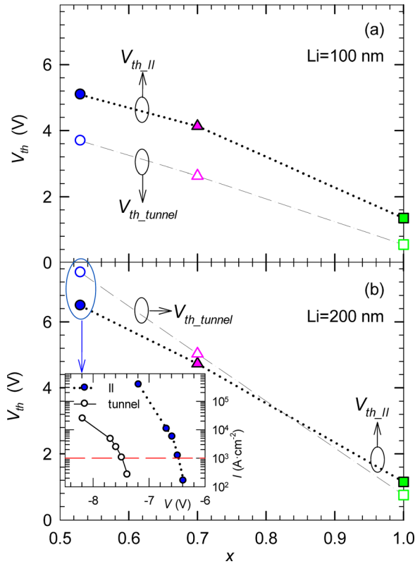
FIG. 2. MC values of V_{th\_II} and V_{th\_tunnel} vs. the In mole fraction x in \text{In}_x\text{Ga}_{1-x}\text{As} (a) 100 nm and (b) 200 nm PIN diodes at room temperature. Inset: MC values of the I-V curves when considering exclusively II processes or band-to-band tunneling in the simulations of an \text{In}_{0.53}\text{Ga}_{0.47}\text{As} 200 nm PIN diode at room temperature.
