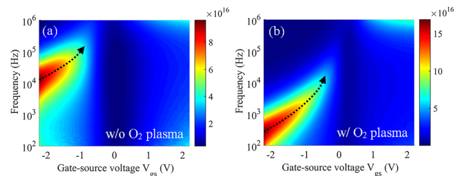
FIG. 2. Conductance map representing magnitude of the normalized parallel conductance as a function of frequency and gate voltage of \text{Al}_2\text{O}_3/\text{n-type In}_{0.53}\text{Ga}_{0.47}\text{As} MOSCAPs (a) without and (b) with the \text{O}_2 plasma postoxidation process. The dotted-line arrow is a guide to the eye to trace the position of the normalized parallel conductance maximum.
