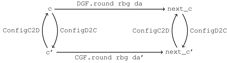
Figure 2. Bisimulation
