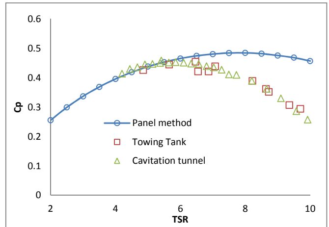
Figure 2. Comparison of power coefficient versus TSR between the potential flow and the experimental results of Bahaj (2007).
