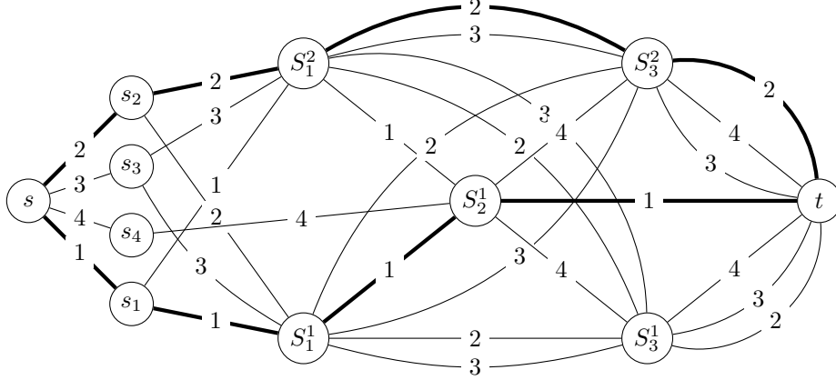
Figure 3: Sample construction of an instance of MAXCDP from an instance of THRESHOLD SET with \mathcal{S} = \{\{1, 2, 3\}, \{1, 4\}, \{2, 3, 4\}\} , w(S_1) = 2, w(S_2) = 1, w(S_3) = 2 . A solution for this instance of THRESHOLD SET could be T' = \{1, 2\} , and we drawn with dark edges the corresponding disjoint paths for MAXCDP.
