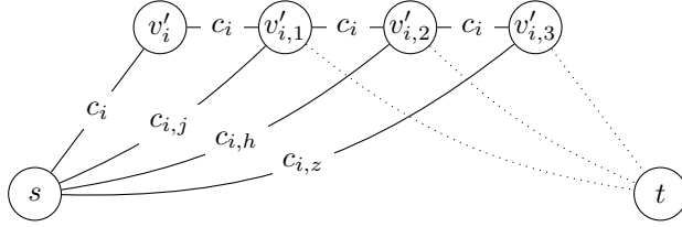
Figure 1: Gadget GV_i associated with vertex v_i \in V_I . Vertices v_j, v_h, v_z are three vertices of V_I , with N(v_i) = \{v_j, v_h, v_z\} and j < h < z . v_j is the first vertex adjacent to v_i in G_I and thus there exists a path in G colored by c_{i,j} that passes through s, v'_{i,1}, t ; v_h is the second vertex adjacent to v_i in G_I (hence there exists a path in G colored by c_{i,h} that passes through s, v'_{i,2}, t ); v_z is the third vertex adjacent to v_i in G_I (hence there exists a path in G colored by c_{i,z} that passes through s, v'_{i,3}, t ).
