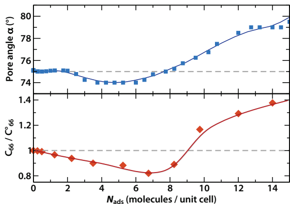
Figure 3. Changes in the lozenge-shaped pore order parameter a (upper frame) and in the elastic constant C_{66} (lower frame) as a function of the number of adsorbed molecules.
