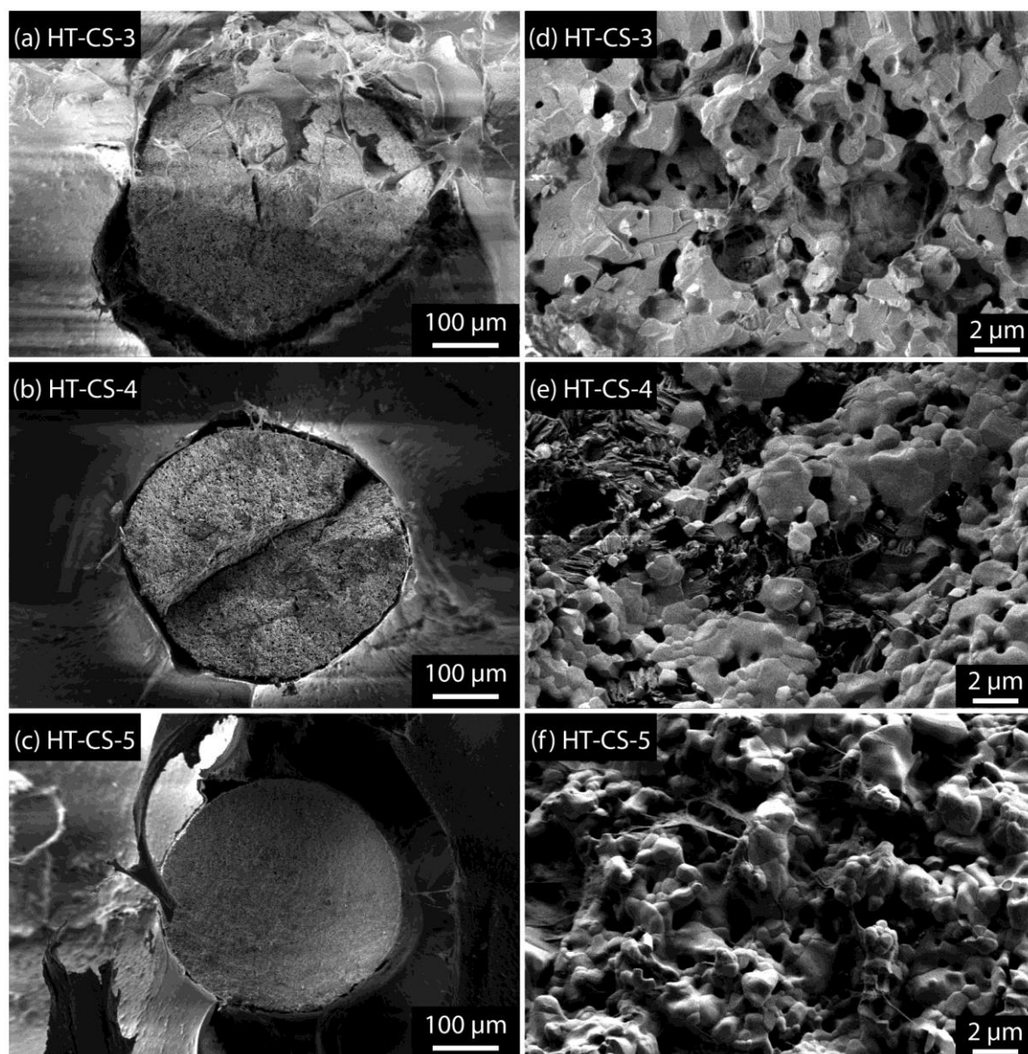
Figure 8: SEM micrographs of HT-CS-3 to HT-CS-5 scaffolds. Column a: cross section of struts; column b: detail of the fracture surface of struts.
