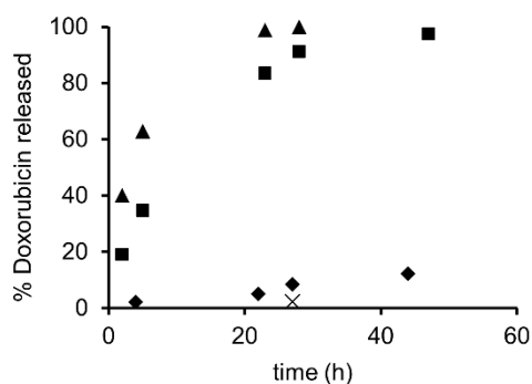
Figure 3. In vitro esterase mediated release of Dox using 100 \mu g/ml esterase in 50 mM Tris buffer (pH 7.4) at 37 ^{\circ} C from LacEsterDox 16 with hCE2(▲), from LacEsterDox 16 with hCE1(◆), from XGOEsterDox 17 with hCE2(■) and LacEsterDox 16 without enzyme (x). The values for hCE2 measurements are mean values of duplicate experiments.
