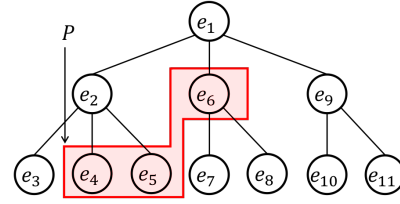
Figure 2: Example of an antichain pattern P = \{e_4, e_5, e_6\}
