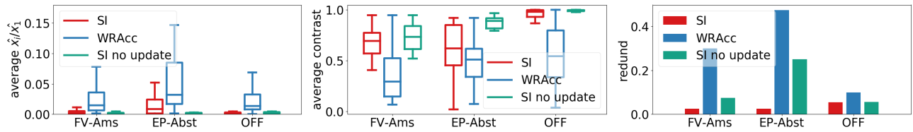
Figure 6: Comparison of (1) normalized supports, (2) contrast, (3) redundancy between the top antichains of the three measures: SI , WRAcc , and SI without model updating.
