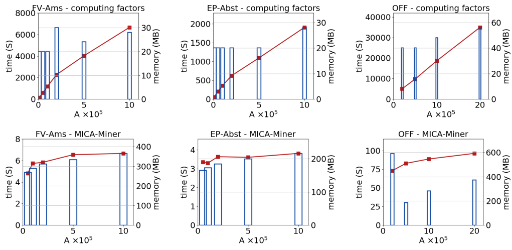
Figure 8: Supplementary experiments. Time (line) and memory consumption (bars) of the factor functions computation (row 1), and MICA-Miner (row 2) in the studied datasets w.r.t. A .
