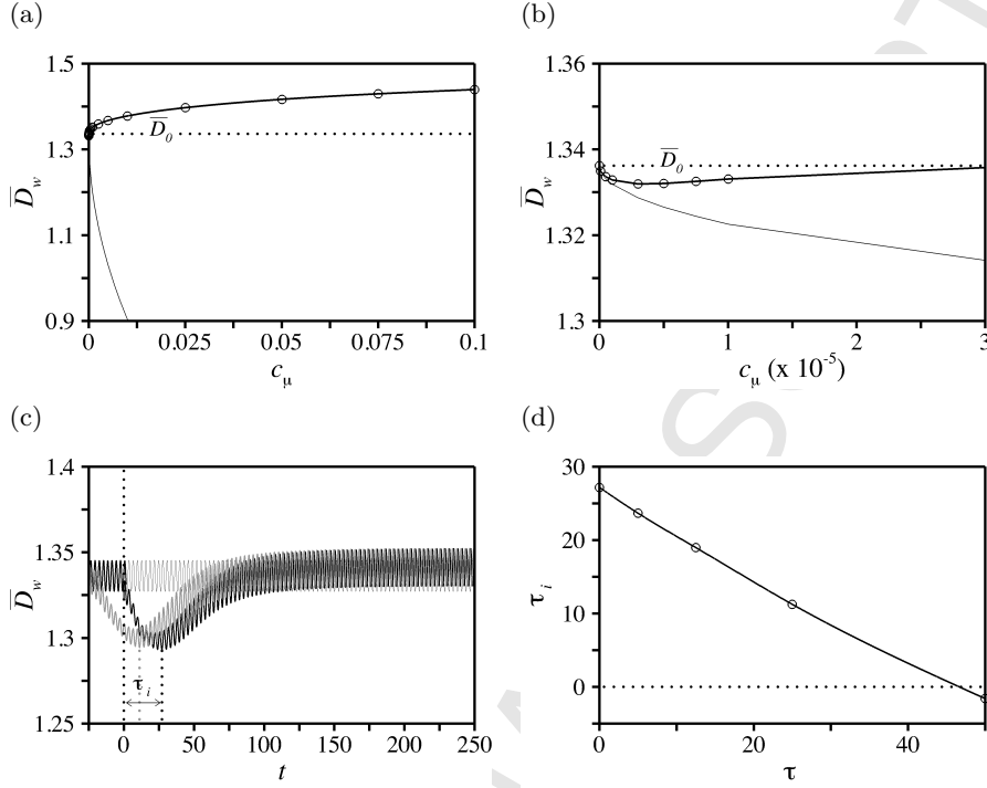
Figure 2: (a) Mean drag of the cylinder flow forced by a control velocity set against the time-dependent sensitivity, i.e., u_w(t, \theta) = -\alpha\zeta(t, \theta) . The solid and dashed lines correspond respectively to the nonlinear value drag computed by DNS, and to the open-loop, linear optimal value computed from Eq. (17) - Re = 100 . (b) Close-up at small control amplitudes. (c) Time evolution of drag for a time-dependent control velocity set against the instantaneous sensitivity. The black line is obtained setting the aerodynamic momentum coefficient to c_\mu = 10^{-4} at t = 0 , as marked by the leftmost vertical dots. The grey line is obtained increasing linearly the coefficient from zero up to 10^{-4} within a time span \tau = 25 , as defined by Eq. (13). The fine line denotes the drag of the uncontrolled cylinder flow - Re = 100 . (d) Time \tau_i after which drag starts to increase against time span \tau used to increase linearly the momentum coefficient from zero.
