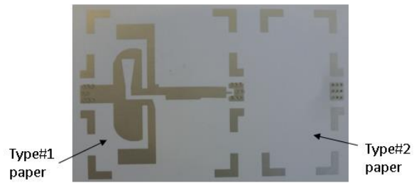
Fig. 5. Realized dual-band printed antenna before assembling.
