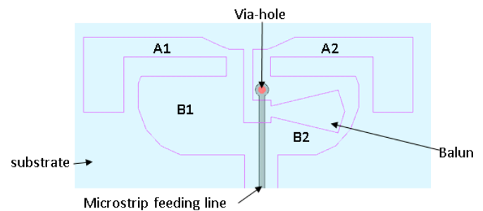
Fig. 1. Original dual-band dipole antenna including a balun.
