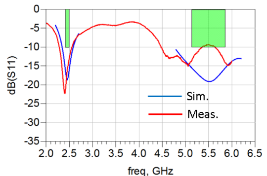
Fig. 7. Simulated and measured reflection coefficient of the dual-band antenna.
