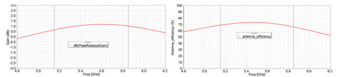
Fig. 14. Simulated peak gain and efficiency of the 5GHz WLAN dipole antenna.
