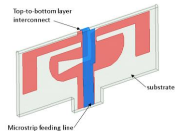
Fig. 2. Dual-band dipole antenna fed directly via an interconnecting line.
