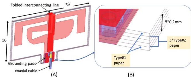
Fig. 3. Paper-based dipole antenna fed with a coaxial cable.
