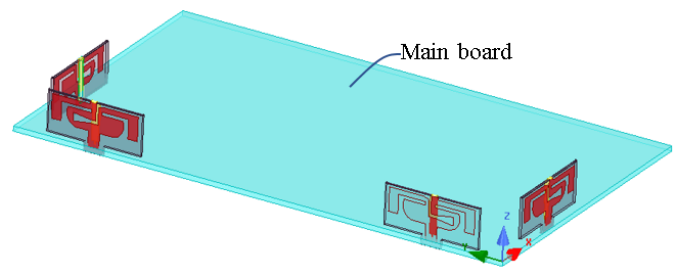
Fig. 12. Example of application of the paper-based dipole antennas in an 4*4 dual-band MIMO system.
