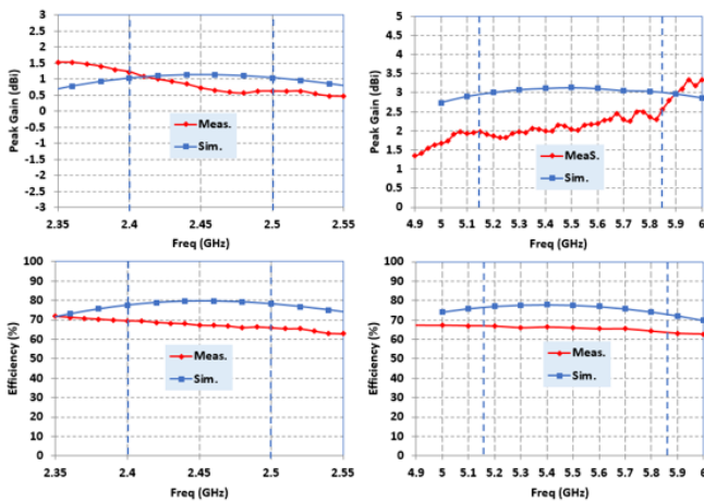
Fig. 9. Simulated and measured peak gain and efficiency of the dual-band antenna.
