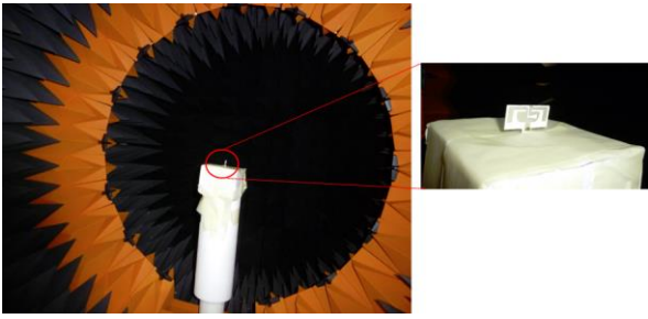
Fig. 8. The dipole antenna measured in near field with a compact StarLab™ measurement tool.
