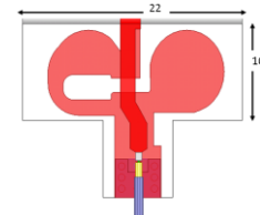
Fig. 13. Paper-based 5GHz WLAN dipole antenna with integrated balun, with the simulated S11 response.
