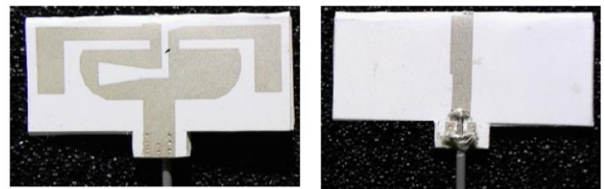
Fig. 6. The whole realized dual-band dipole antenna fed by a coaxial cable.
