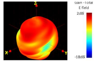
Fig. 11. Measured 3D radiation pattern of dipole antenna at 5.5GHz.
