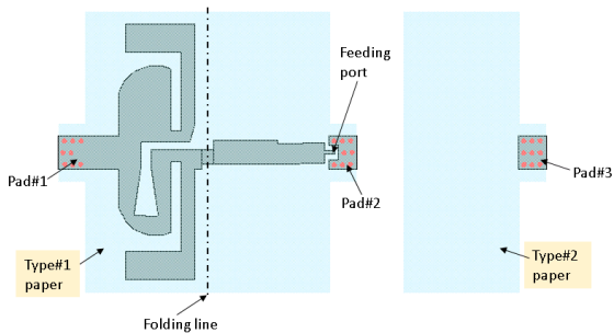
Fig. 4. Constituent parts of the multilayer paper-based antenna.
