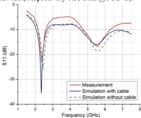
Fig. 4 Return loss S_{11} of this dual-band Wi-Fi monopole antenna
