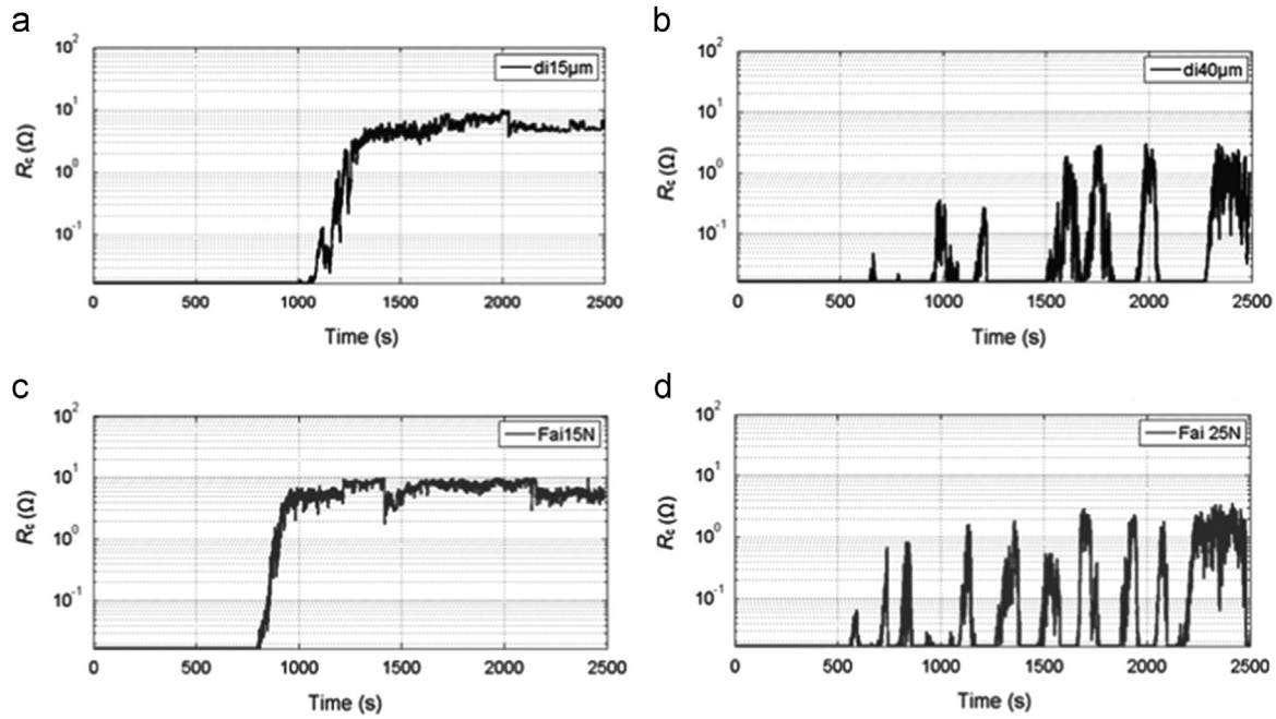
Fig. 22. Temporal evolution of the electrical resistance of a CuSn6–CuSn6 contact (a) at imposed displacement ( \delta_i \pm 15 \mu\text{m} ), (b) at imposed displacement ( \delta_i \pm 40 \mu\text{m} ), (c) at imposed force ( F_{ai} \pm 15 \text{N} ), and (d) at imposed force ( F_{ai} \pm 25 \text{N} ), I = 100 \text{mA} , F_N = 6 \text{N} , f = 10 \text{Hz} , N_c = 25,000 cycles.
