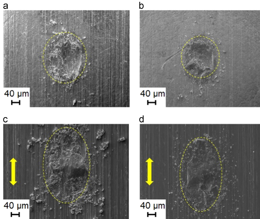
Fig. 16. Wear track observations by SEM: (a) CuSn6 hemispherical slider and (b) CuSn6 flat sample for imposed displacement tests at \delta_i \pm 40 \mu\text{m} ; (c) CuSn6 hemispherical slider and (d) CuSn6 flat sample for imposed actuator force test ( F_{ai} \pm 15 \text{ N} ), with F_N = 1 \text{ N} , f = 10 \text{ Hz} , N_c = 400 cycles.
