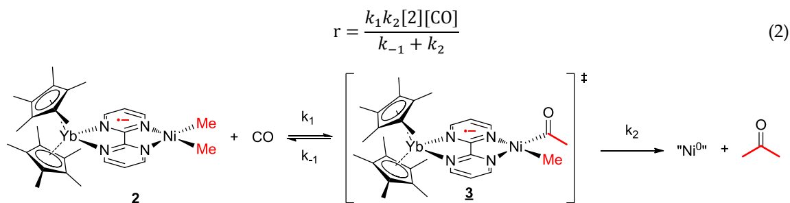
Scheme 3. Mechanism for the reaction of 2 with CO.
