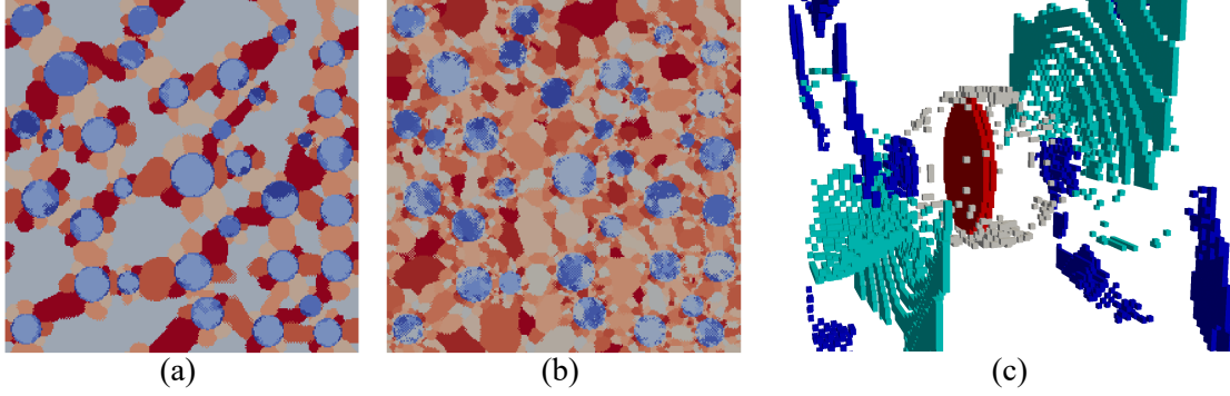
Figure 2: Ductile materials' microstructures: (a) two-dimensional microstructure discretized using 8 clusters, (b) same two-dimensional microstructure discretized using 65 clusters, (c) three-dimensional microstructure discretized using 217 clusters showing two clusters in the matrix phase (two shades of blue), one cluster in the inclusion phase (red), and one cluster in the void phase (light gray).
