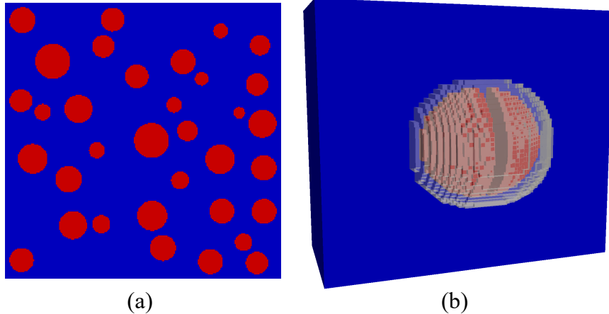
Figure 1: Ductile materials' microstructures discretized using voxel meshes with matrix shown in blue and inclusions in red: (a) two-dimensional microstructure, (b) inside view of a three-dimensional microstructure with a fragmented inclusion surrounded by a debonding void shown in light gray.
