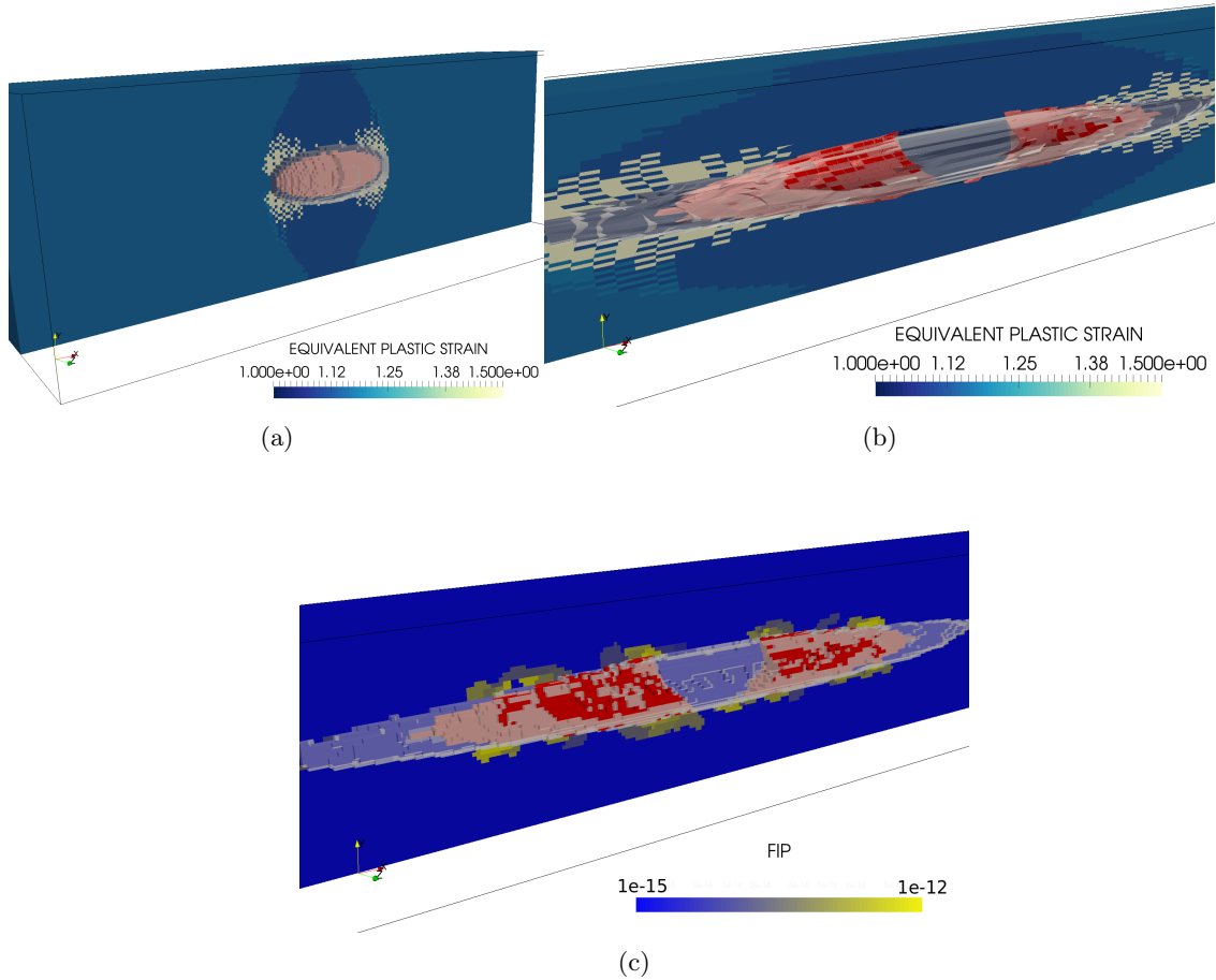
Figure 6: Cold drawing and FIP computation results showing the particle fragments in red, the voids in light gray, and: (a) the equivalent plastic strain in the matrix in undeformed configuration, (b) the equivalent plastic strain in the matrix in deformed configuration after displacement reconstruction, (c) the FIP in the matrix on a new voxel mesh of the deformed configuration after mesh transfer. Note that the three figures are not in the same spatial scale, as section height in (b,c) is reduced by 45% compared to (a).
