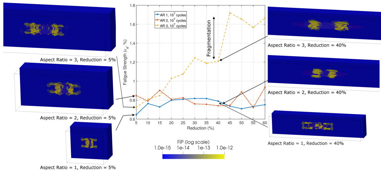
Figure 7: Fatigue strength at 10^7 cycles as a function of cold drawing section reduction for 1:1:1, 2:1:1, and 3:1:1 initial AR (x:y:z). Fragmentation occurs between 40% and 45% reduction for AR 3, resulting in a jump in fatigue strength
