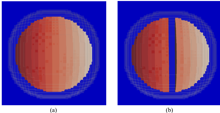
Figure 5: Clusters (shades of red) within the debonded inclusion: (a) before fragmentation, (b) after fragmentation with the missing cluster turned into void. Drawing direction is horizontal.
