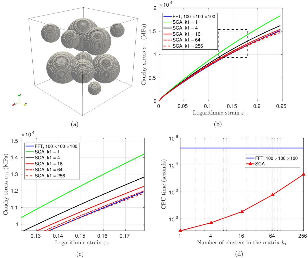
Figure 3: (a) Ductile composite with particle volume fraction of 20%; (b) SCA converges fast to the FFT reference for the overall mechanical response of the RVE under unidirectional tension along the x direction; (c) a closer look at the dashed rectangle area in (b) shows accurate prediction of SCA with only 16 clusters; (d) a CPU time saving of a factor of more than 10^3 is achieved with SCA for the relatively well-converged number of clusters, compared with the FFT reference with a 100 \times 100 \times 100 voxel mesh.
