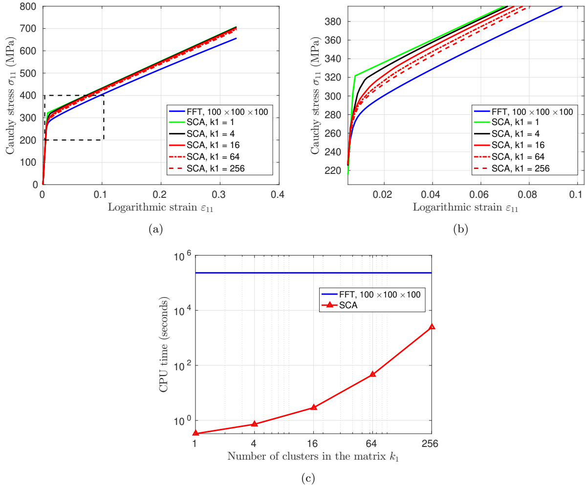
Figure 4: (a) SCA is fairly close to the FFT reference for the overall mechanical response of the porous RVE under uniaxial tension along the x direction; (b) a closer look at dashed rectangle area in (a) shows the relatively slow convergence; (c) a CPU time saving of a factor of more than 10^3 is achieved with SCA for relatively well-converged numbers of clusters, compared with the FFT reference with a 100 \times 100 \times 100 voxel mesh.
