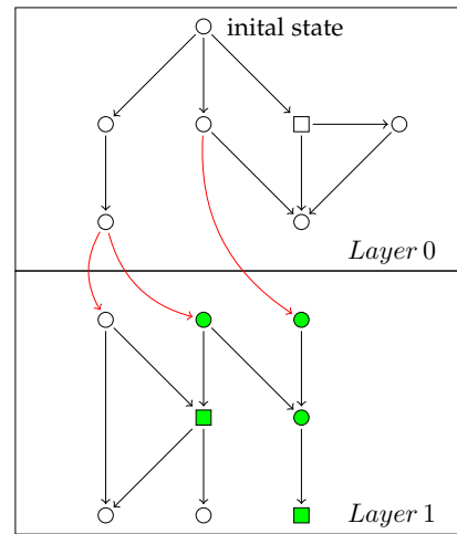
Fig. 4: Computing W_1 = \text{bas}(\psi_1) , in green.
