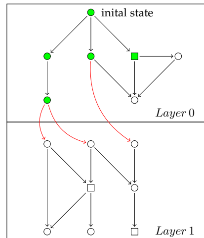
Fig. 6: Computing in green W_0 = \text{bas}(\psi_0) .
