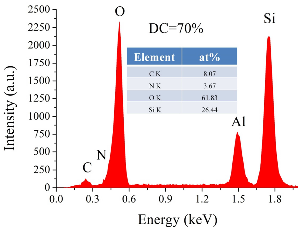
Supplemental material 6: EDX analyses of powders collected on an aluminium substrate for duty cycles equal to 20 and 70%. (P = 15 mbar, W = 250 W, flowrates: Ar =1050 sccm, O 2 = 100 sccm, Ar =30 sccm, APTES = 0.13 sccm)
