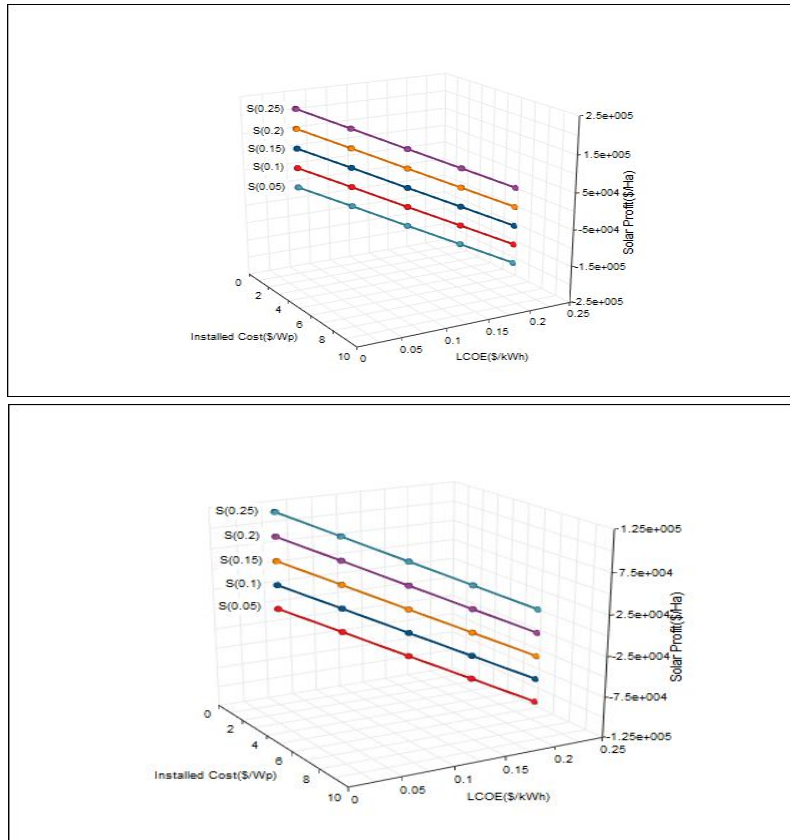
Figure 8. Effect of electricity cost and installed costs on the solar profit for full density (8A), ground mount (8B) and half density (8C), configurations respectively.
