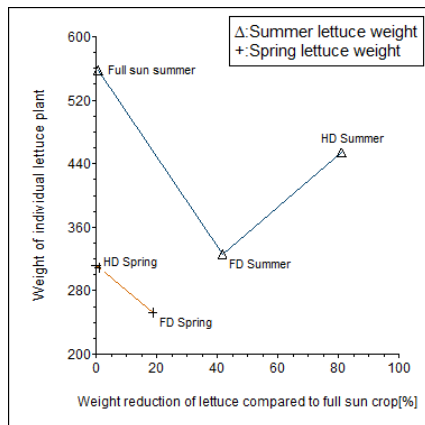
Figure 5. Sensitivity of lettuce plant weight with respect to change in shading values for agrivoltaic farm configurations.
