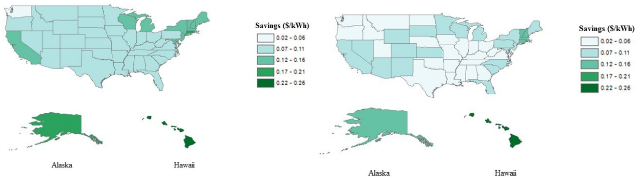
Figure 2 Prosumer savings obtained by installing the solar plug and play system at A) 1% and B) 7% discount rate respectively. Assumptions- the capital cost of the system is considered as $1.25/W and life span of the system is 25years with 0.5%/year degradation rate and current electricity rates for residential sector.
