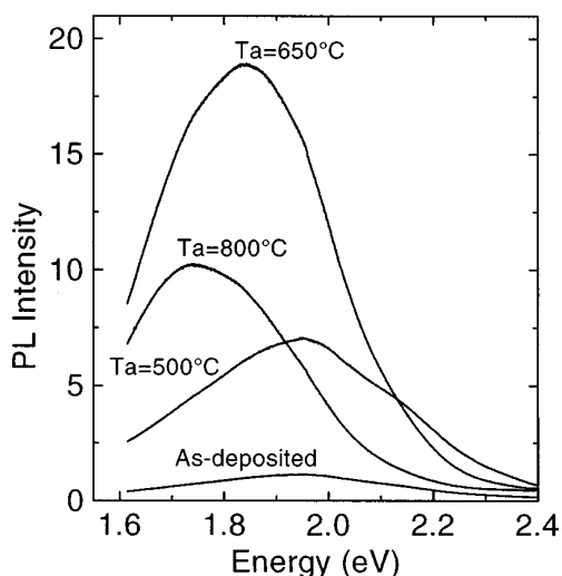
FIG. 4. Photoluminescence spectra of a\text{-SiO}_x\text{:H} films annealed at different temperatures T_a .
