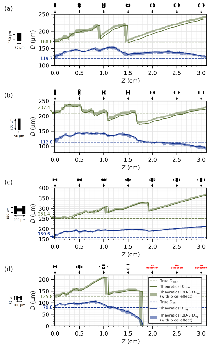
Figure 8. Evolution of the theoretical D_{eq} (solid blue line) and D_{max} (solid green line) of the diffracting image of a particle as a function of Z (with a 50 % intensity threshold), compared to the true D_{eq} (dashed blue line) and the true D_{max} (dashed green line) of the particle. Binary images from diffraction patterns added on top of four figures for several Z distances. Blue and green shadow areas are the theoretical records by the 2D-S with the uncertainty due to the position of the particle in front of the photodiode array. Only 0^\circ particle orientation is considered here.
