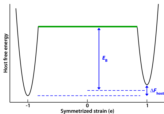
Figure 2: Schematics of the host free energy landscape for the “dry” bistable framework, as a function of symmetrized strain e . Two regions of elastic deformation around the equilibrium lp and np structures ( e = \pm 1 )
