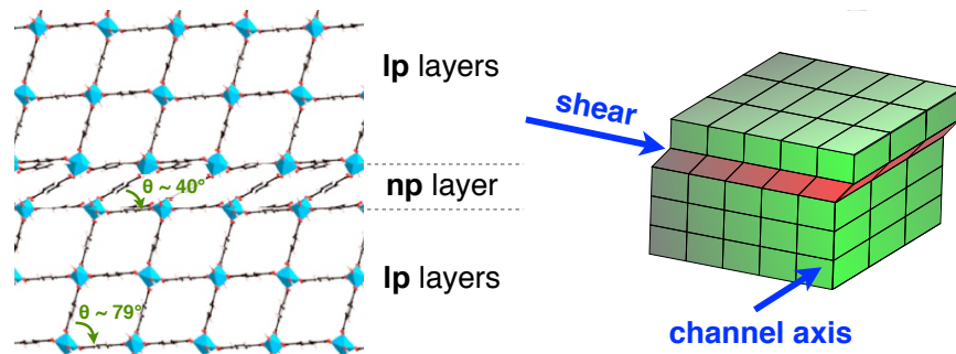
Figure 1. Schematic representation of the MIL-53 framework after the first event of lp-np transformation, which involves in-plane shear of a 2D layer of cells in a direction orthogonal to the channel axis.
