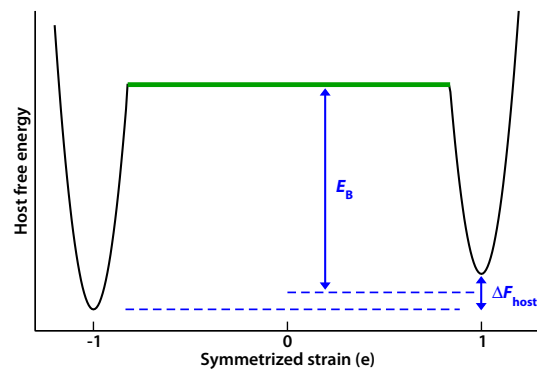
Figure 2: Schematics of the host free energy landscape for the “dry” bistable framework, as a function of symmetrized strain e . Two regions of elastic deformation around the equilibrium lp and np structures ( e = \pm 1 )
