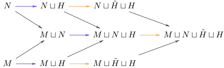
FIGURE 4. In this diagram, orange arrows correspond to the coproduct of H . We see the map (\text{id}_{M \sqcup N} \sqcup \Delta) \circ \Omega_{M \sqcup N} in the middle line.
