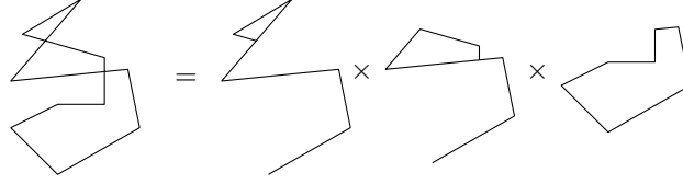
FIGURE 27. Decomposition of a loop into a product of lassos.
