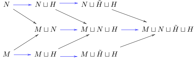
FIGURE 3. This diagram, in which blue arrows correspond to the coaction of H , shows the map (\Omega_{M \sqcup N} \sqcup \text{id}_H) \circ \Omega_{M \sqcup N} .
