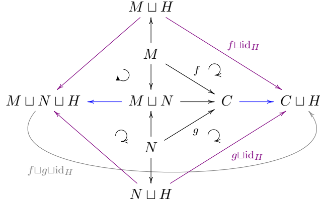
FIGURE 5. Equivariance of the map f \dot{\cup} g . The morphisms drawn in violet and gray are equal to the morphisms drawn with the same colour in Figure 6.
