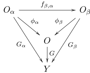
FIGURE 25. Universal property of the inductive limit.
