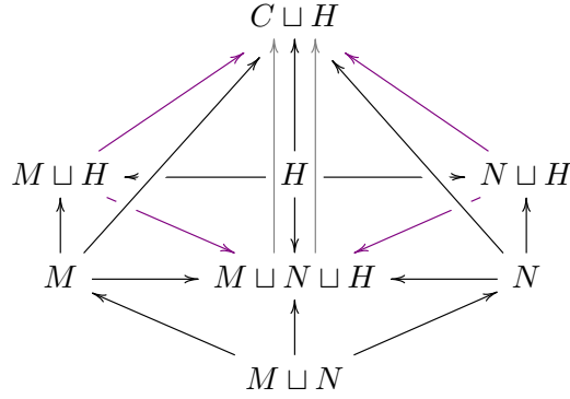
FIGURE 5. Equivariance of the map f \dot{\cup} g . The morphisms drawn in violet and gray are equal to the morphisms drawn with the same colour in Figure 6.
