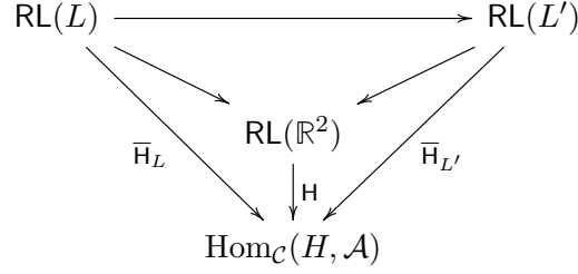
FIGURE 28. The holonomy H obtained as a solution of an universal problem.
