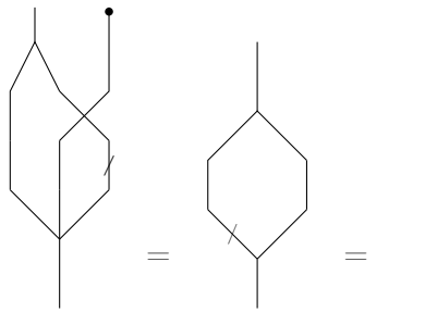
FIGURE 16. Diagrammatic proof of the relation \eta_H \circ \epsilon = (\text{id}_H \sqcup \epsilon) \circ \Omega_c .
