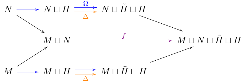
FIGURE 2. In this diagram, blue arrows indicate a coaction of H and orange arrows a coproduct of H . We use the notation \tilde{H} for the sake of clarity.
