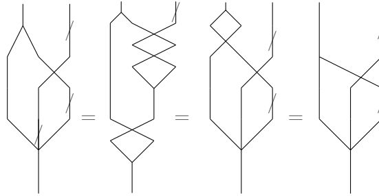
FIGURE 15. The relation S \circ \Omega_c = (\text{id}_H \sqcup S) \circ \Omega_c .
