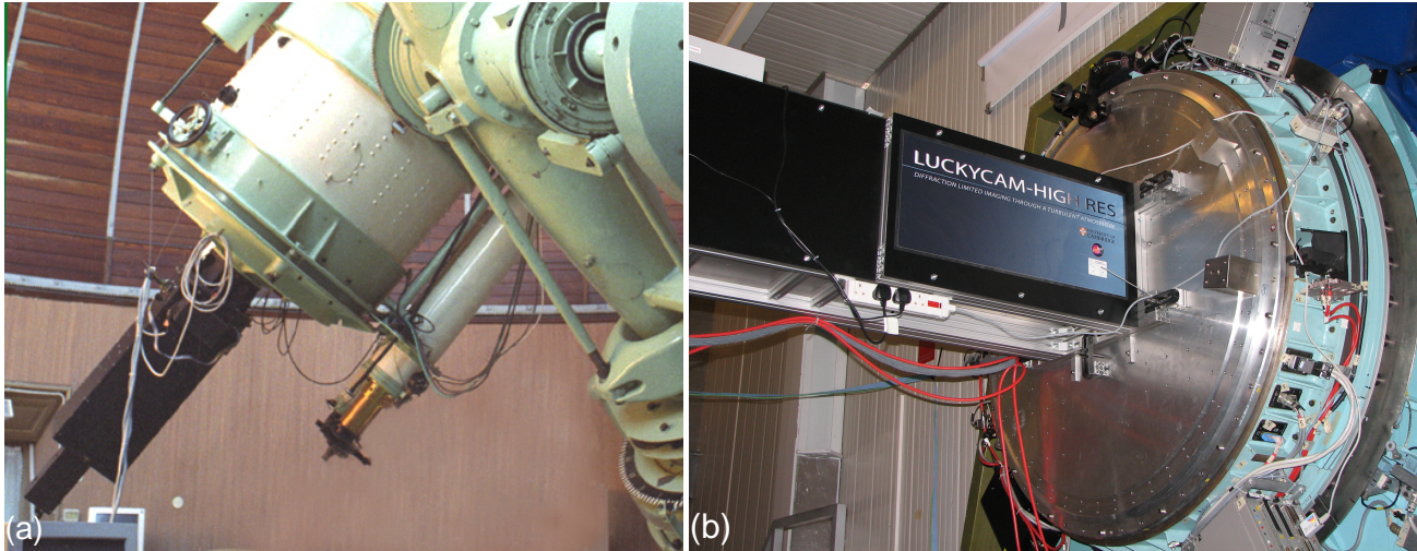
Fig. 1 PISCO on the Zeiss telescope in Merate (a) and LuckyCam at the Nasmyth focus of the ESO NTT (b).
