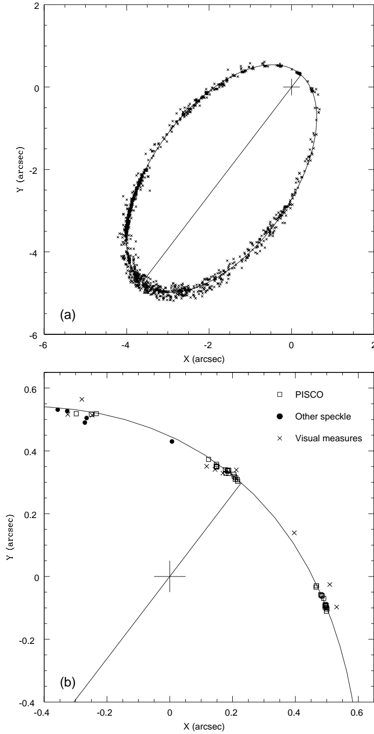
Fig. 2 The apparent orbit of \gamma Vir (a) and enlarged view around periastron (b) (North to the bottom, East to the right).
