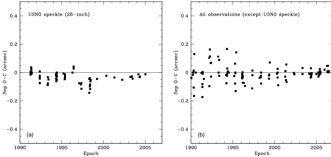
Fig. 4 Orbital residuals in separation for the period 1990–2006: USNO speckle measurements only (a) and other measurements (b).
