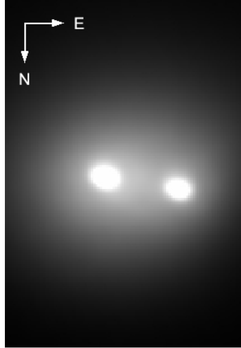
Fig. 6 Unsharp masked SDSS i' -band image of \gamma Vir A and B obtained with LuckyCam on the 3.6m ESO NTT on June 5th 2006, when the angular separation was 0''.5 .
