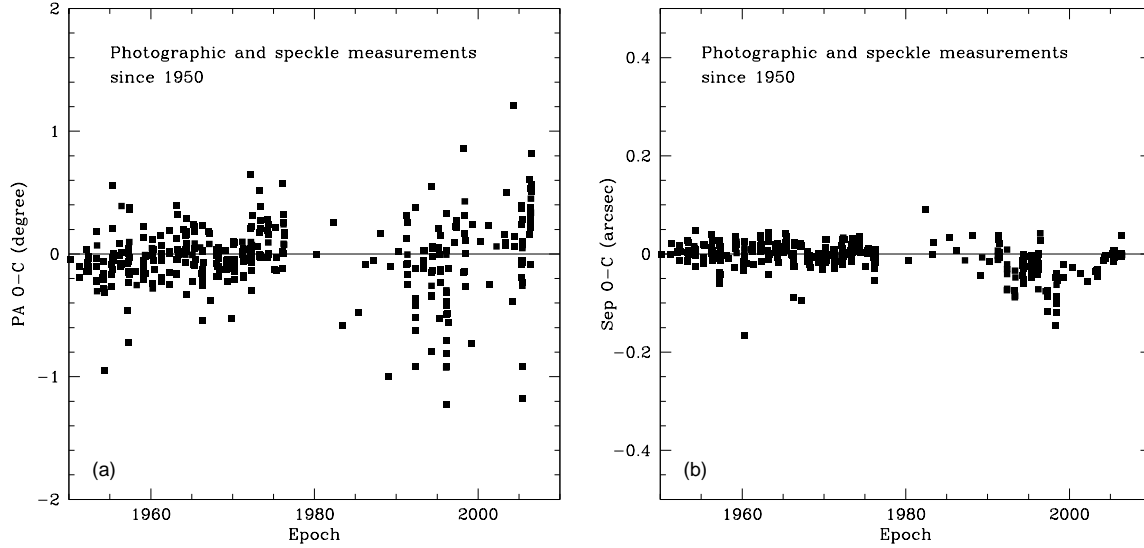
Fig. 3 Orbital residuals in position angle (a) and in separation (b) for the period 1950–2006.
