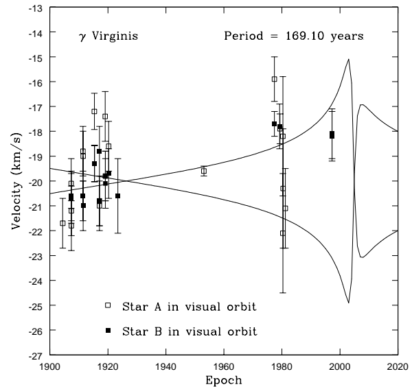
Fig. 5 Observed individual radial velocities and predicted velocity curves.
