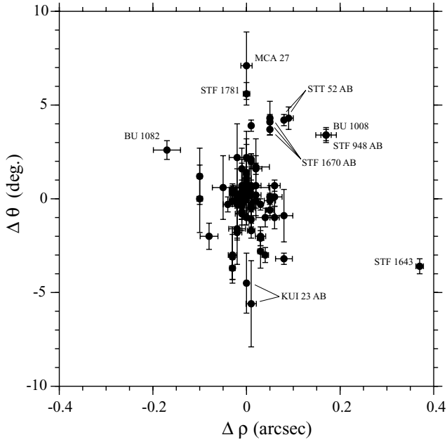
Figure 2. Residuals with published orbits.
