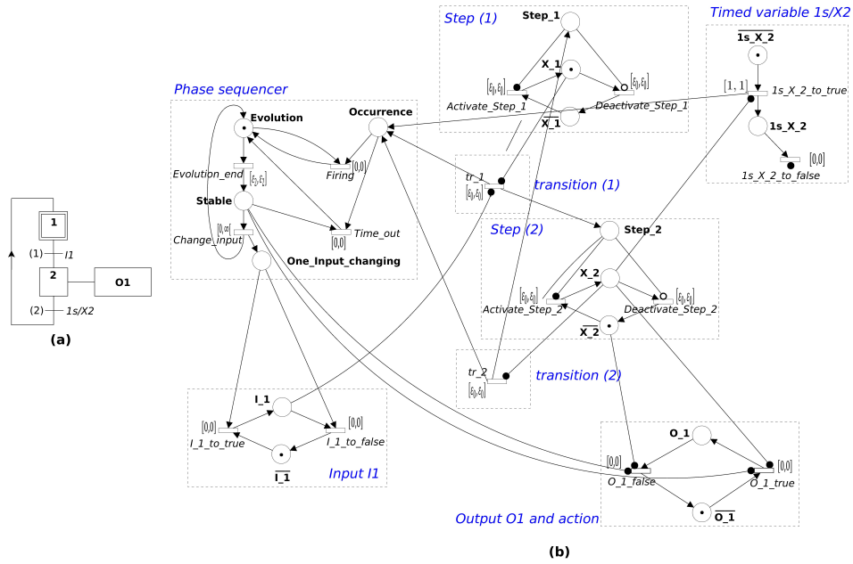
Figure 5. The example of grafset at Fig. 1 (a) and the translation into \epsilon -TPN (b).
