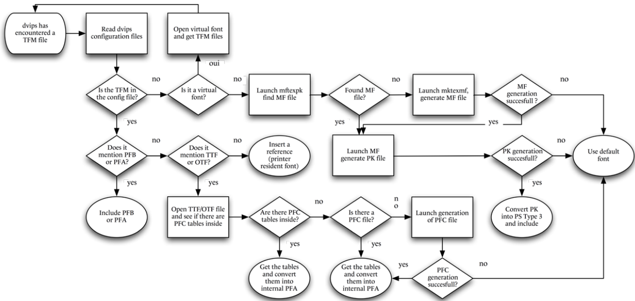
Figure 1: dvips responding to a font request in the DVI file.
