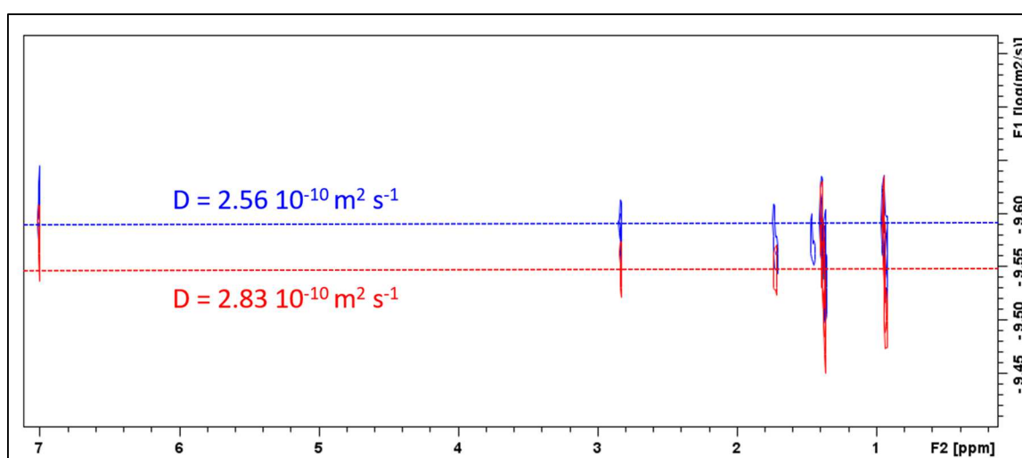
Fig. 2. ^1\text{H} NMR-DOSY spectra of the P3HT- b -PFPE- b -P3HT triblock copolymer (blue) and ethynyl end-functionalized P3HT precursor (red) recorded in CDCl 3 at 25 °C.
