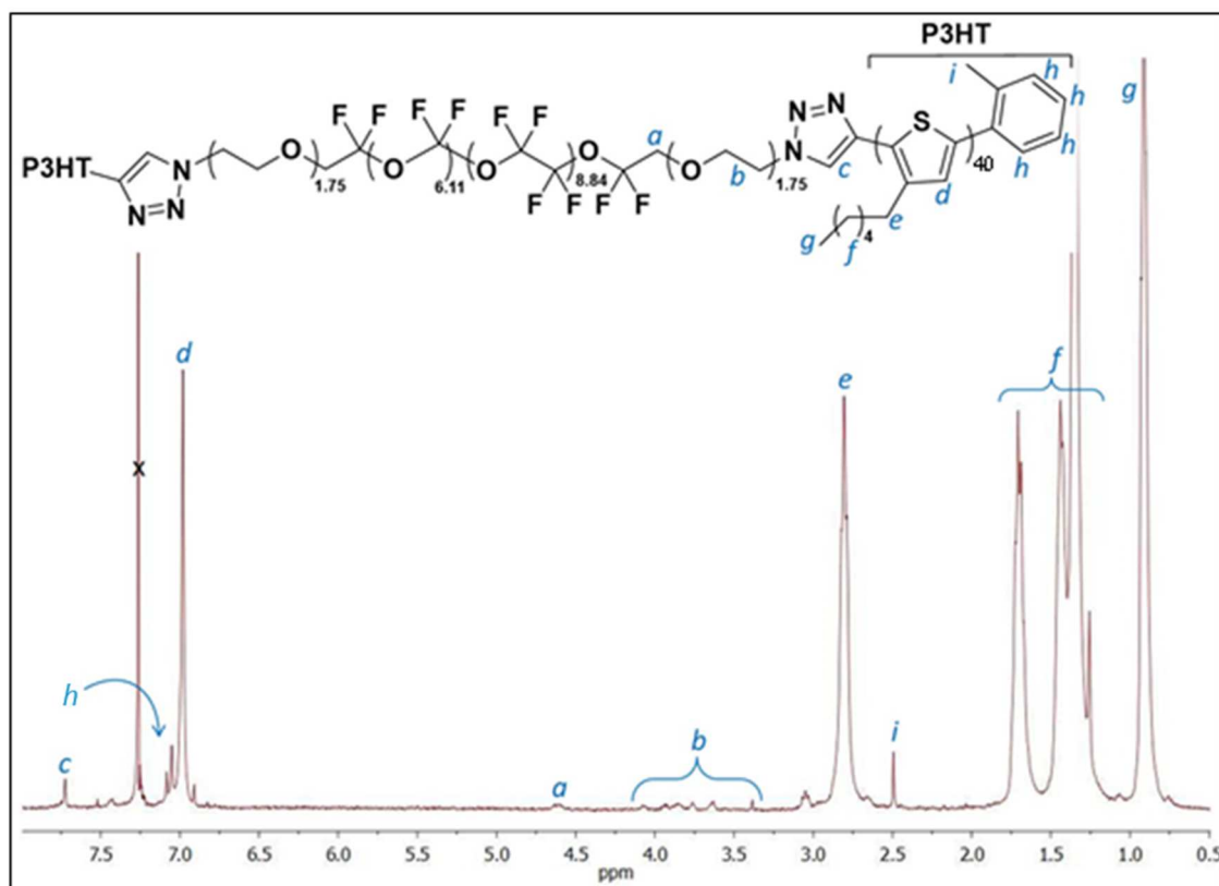
Fig. 1. ^1\text{H} NMR spectrum of the P3HT- b -PFPE- b -P3HT triblock copolymer in \text{CDCl}_3 at 25^\circ\text{C} .
