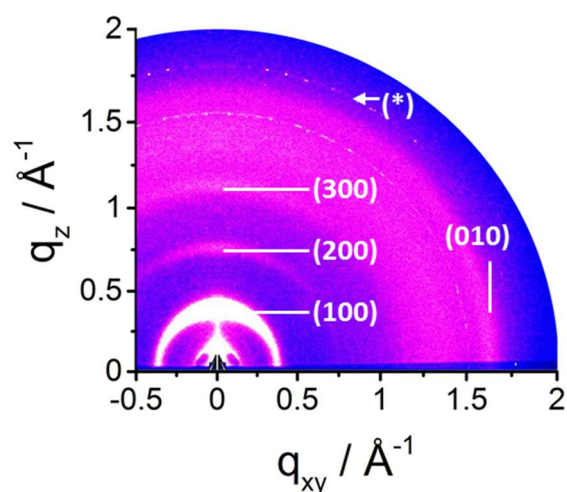
Fig. 3. GIWAXS pattern of the P3HT- b -PFPE- b -P3HT film. Reflections are assigned by using Miller indexes. (*) Artefact.
