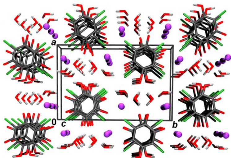
Figure 5 Crystal packing of \text{KHCA}\cdot 2\text{H}_2\text{O} viewed approximately along the direction [001] . Potassium cations are shown as spheres of arbitrary radii.
